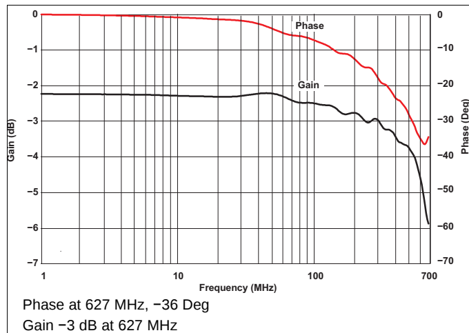
Figure 1. Gain and Phase vs Frequency
