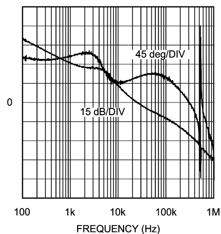
Figure 5. Overall Loop Gain and Phase ( f_o = 500 \text{ kHz} , V_{IN} = 12V , V_{OUT} = 3.3V , I_{OUT} = 2A )
