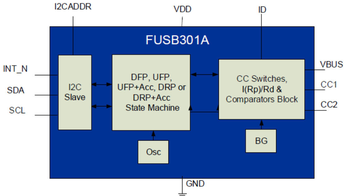
Figure 2. Block Diagram
