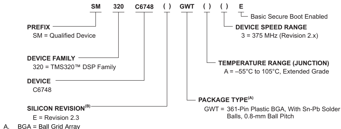
Figure 6-1. Device Nomenclature
