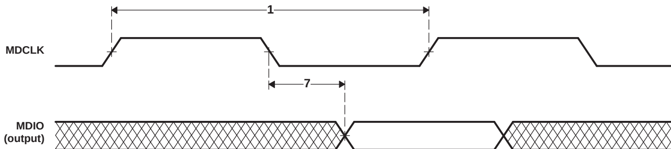
Figure 4-54. MDIO Output Timing
