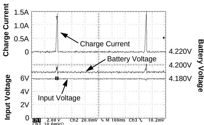
Figure 2. Waveforms showing overcurrent protection
