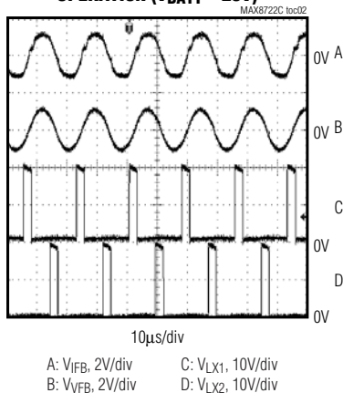
HIGH INPUT-VOLTAGE OPERATION ( V_{BATT} = 20V )
