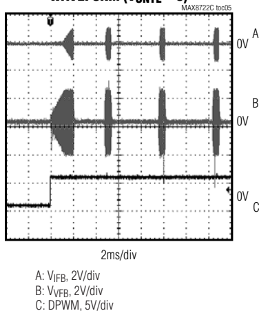
MINIMUM BRIGHTNESS STARTUP WAVEFORM ( V_{CNTL} = 0 )
