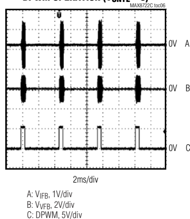
MINIMUM BRIGHTNESS DPWM OPERATION ( V_{CNTL} = 0 )
