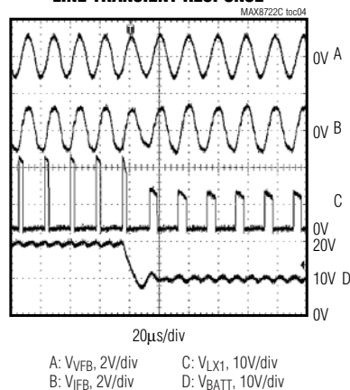
LINE TRANSIENT RESPONSE
