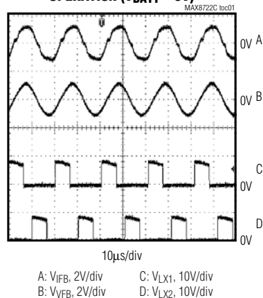
LOW INPUT-VOLTAGE OPERATION ( V_{BATT} = 8V )
