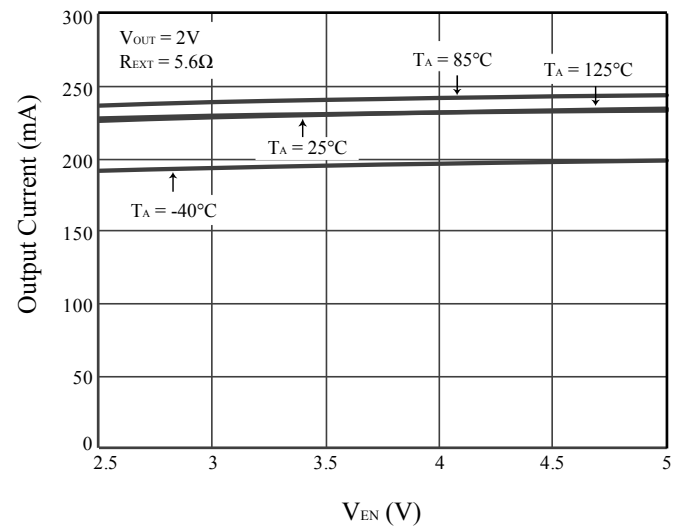
Figure 28 I_{OUT} vs. V_{EN}
