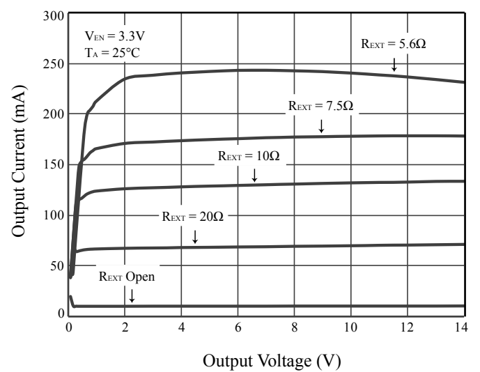
Figure 22 I_{OUT} vs. V_{OUT}
