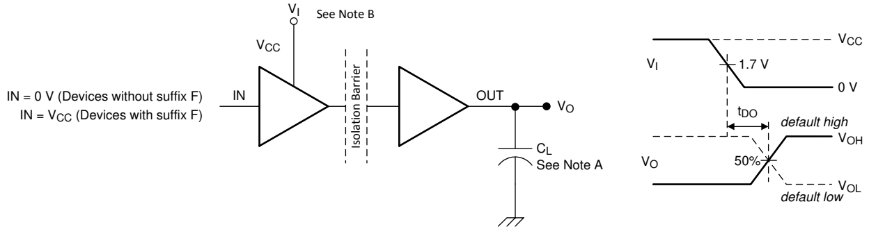
Figure 19. Default Output Delay Time Test Circuit and Voltage Waveforms
