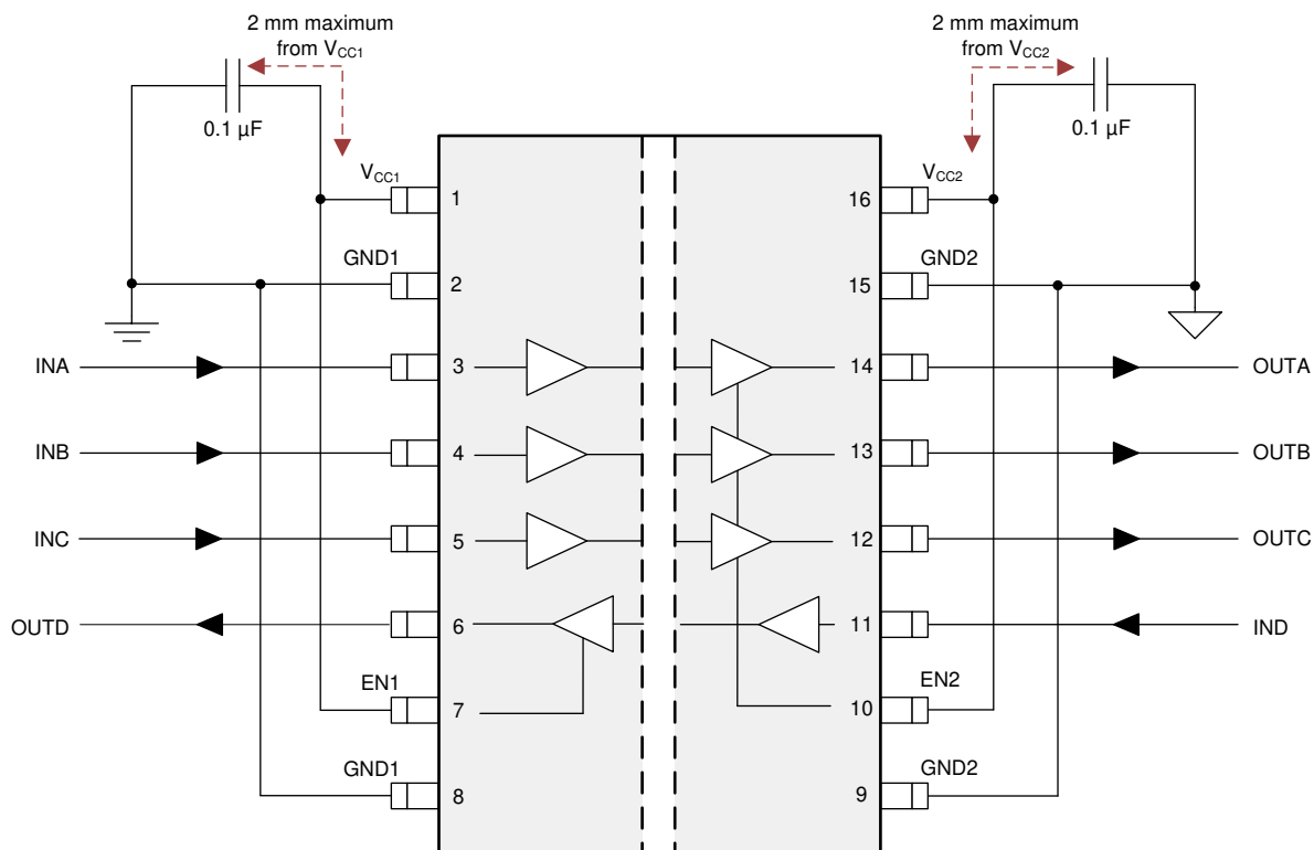
Figure 25. Typical ISO774x-Q1 Circuit Hook-up
