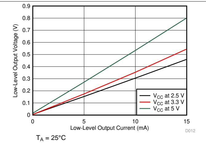
Figure 14. Low-Level Output Voltage vs Low-Level Output Current
