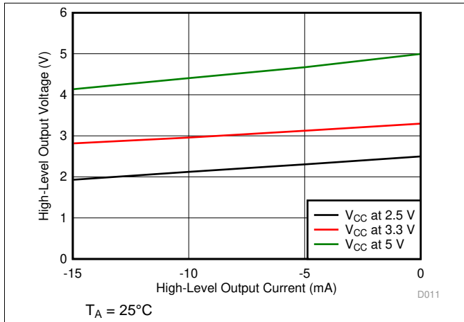
Figure 13. High-Level Output Voltage vs High-level Output Current
