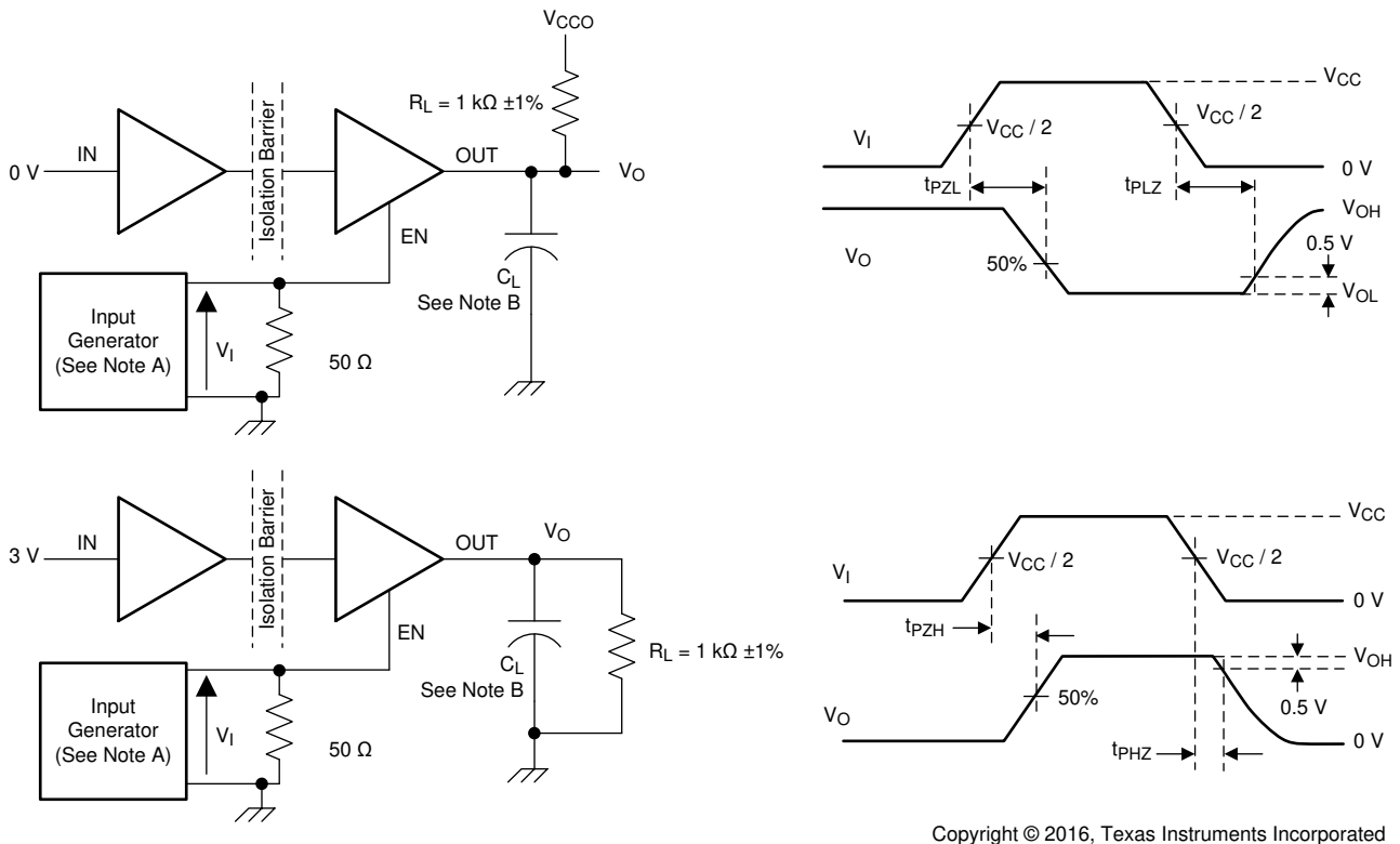
Figure 17. Switching Characteristics Test Circuit and Voltage Waveforms
