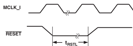
Figure 2. \overline{RESET} Timing
