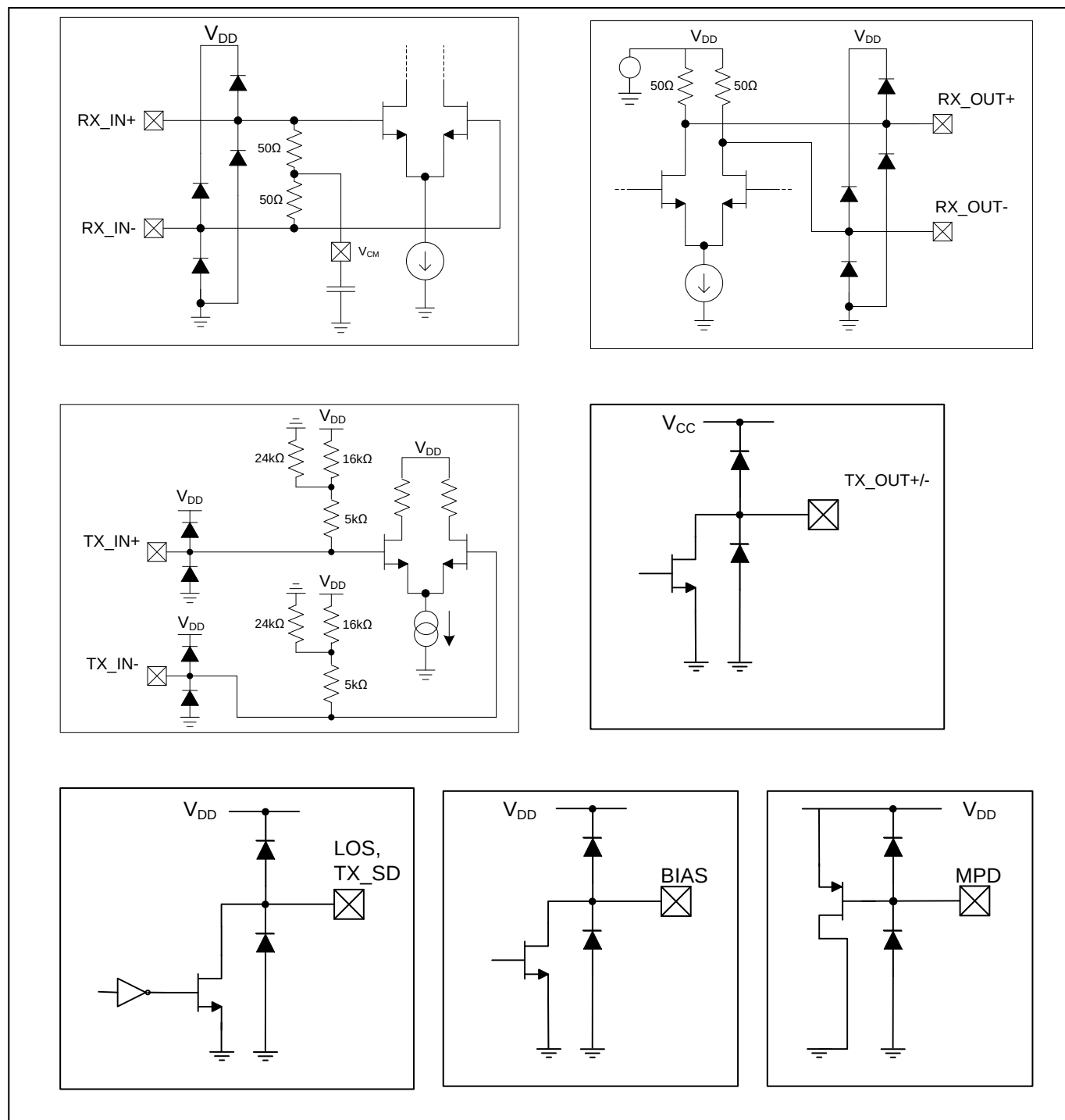
Figure 27. Interface Diagrams
