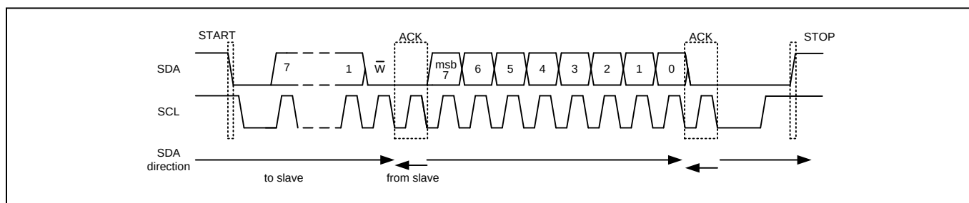
Figure 25. Write Transaction
