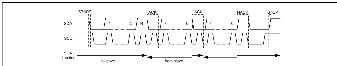
Figure 26. Read Transaction
