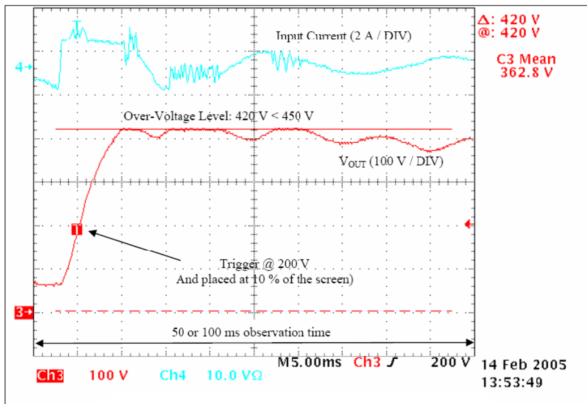
Figure 15. Over-Voltage Protection (Start-Up Sequence @ 220 V_{AC} )
