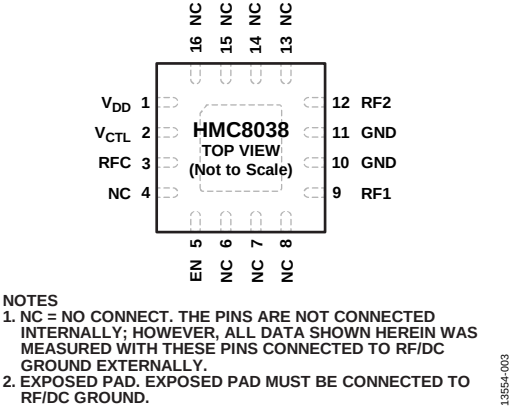
Figure 3. Pin Configuration
