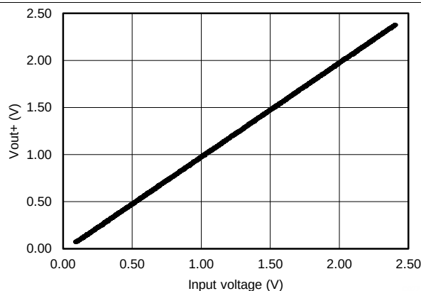
Figure 38. V_{OUT+} vs Input Voltage
