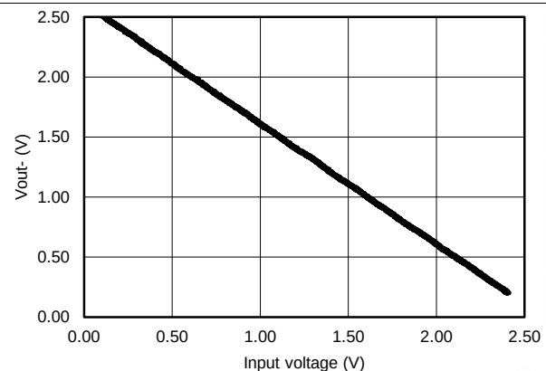
Figure 39. V_{OUT-} vs Input Voltage
