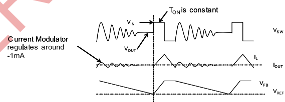
Figure 3—Light Load Operation
