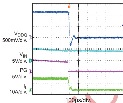
Power Good through Vin Shutdown I_O = 10A
