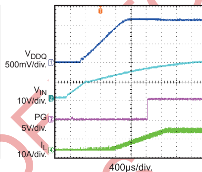
Power Good through Vin Start-up I_O = 10A
