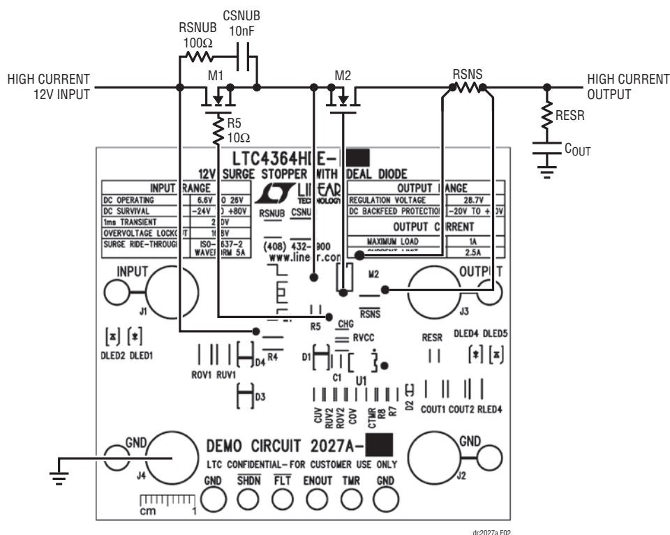
Figure 2. Connections to an Off-Board Power Stage. Remove M1, M2, RSNS, RSNUB and RESR from Board. Keep Wires Short to Avoid Parasitic Oscillations in M1
