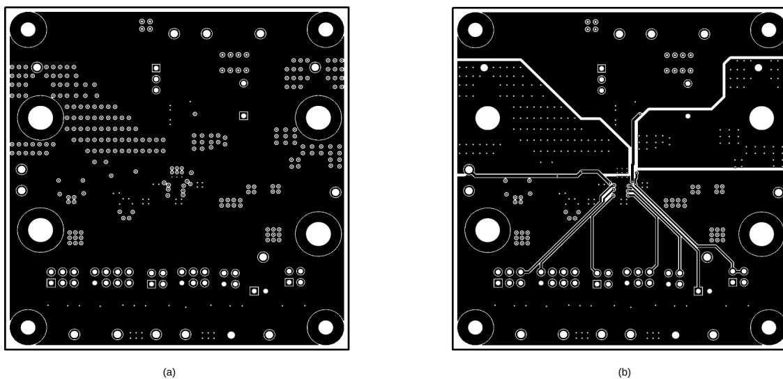
Figure 9. TPS259827LEVM Board (a) Inner Signal Layer (b) Inner Routing Layer
