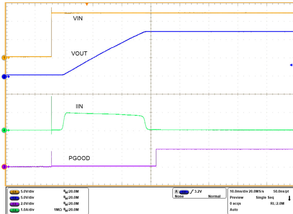
Figure 3. TPS259827L Output Rise Profile (VIN = 12 V, CdVdT = 10 nF, COUT = 2 mF, No-load)
