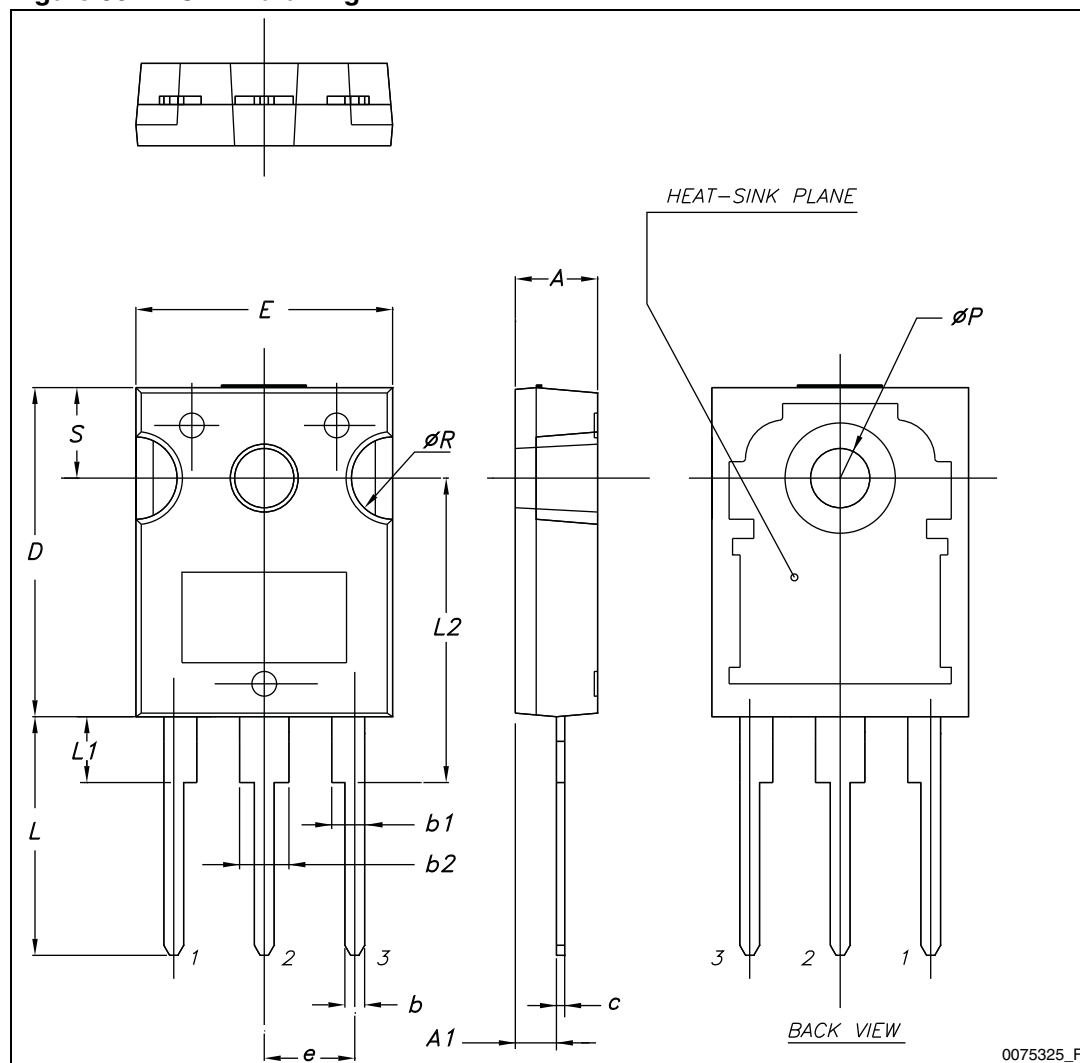
Figure 30. TO-247 drawing
