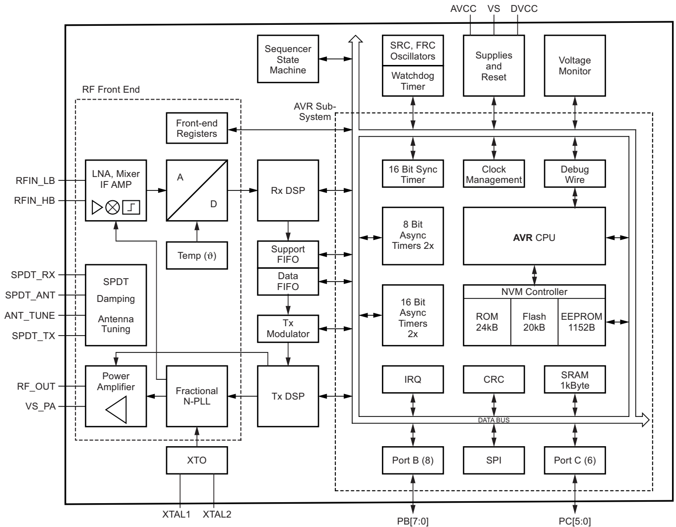
Figure 3-1. Block Diagram
