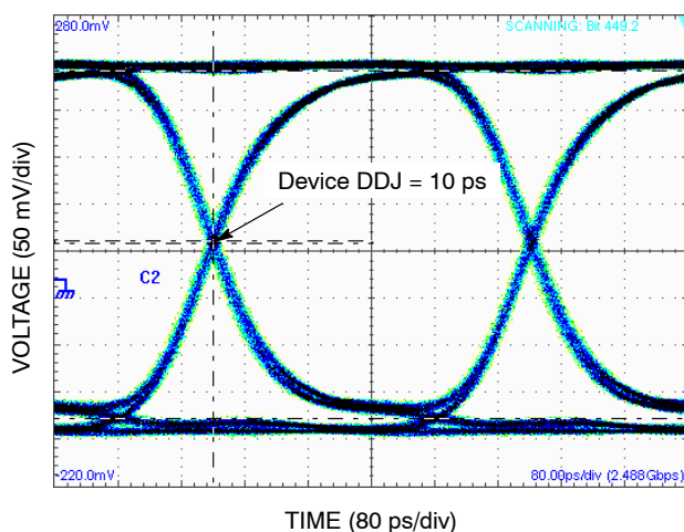
Figure 5. Typical Output Waveform at 2.488 Gb/s with 2^{23}-1 (V_{INPP} = 100 \text{ mV (left) \& } V_{INPP} = 400 \text{ mV (right), Input Signal DDJ = 30 ps)}
