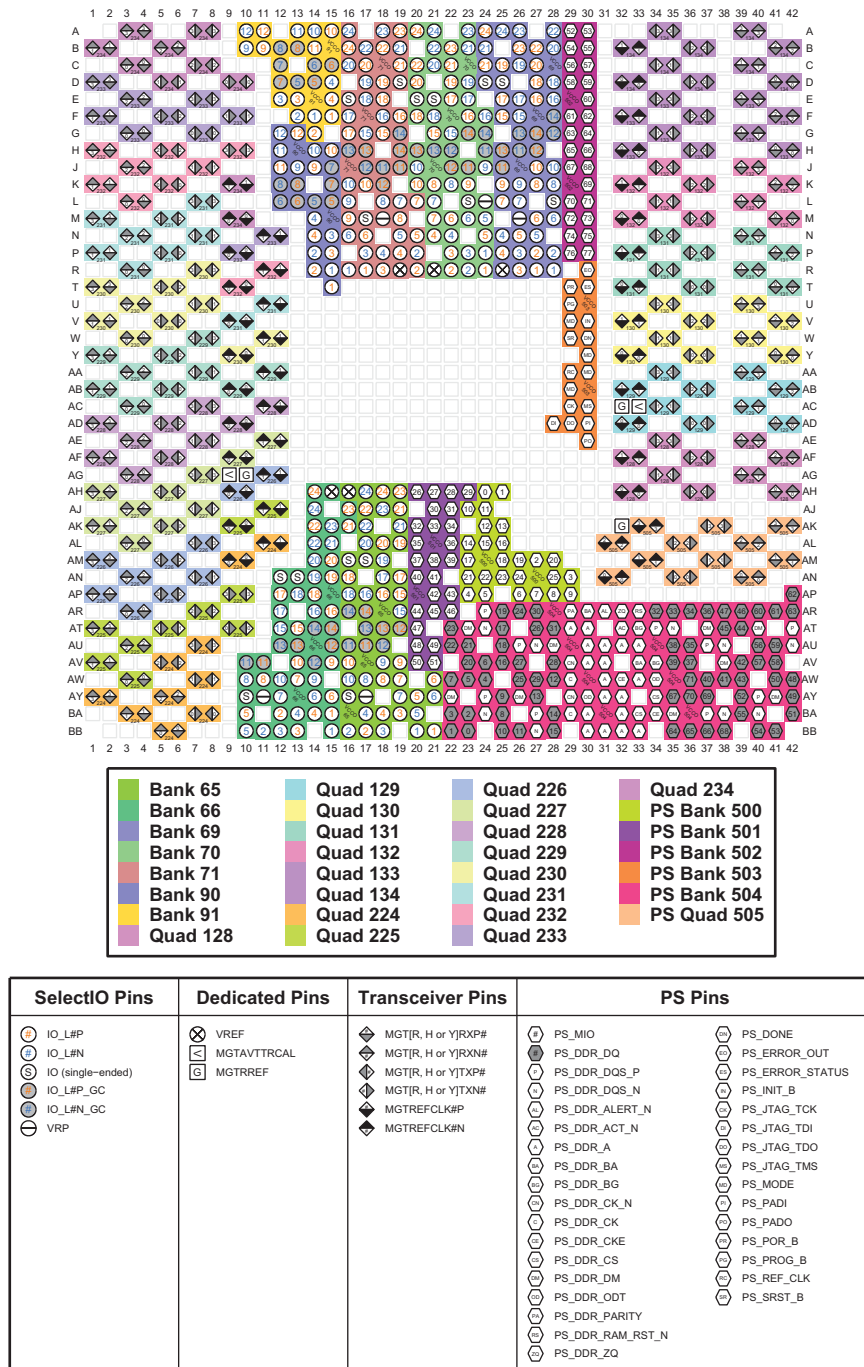
Figure 4-65: FFVD1760 Package—XCZU17EG and XCZU19EG I/O Bank Diagram
