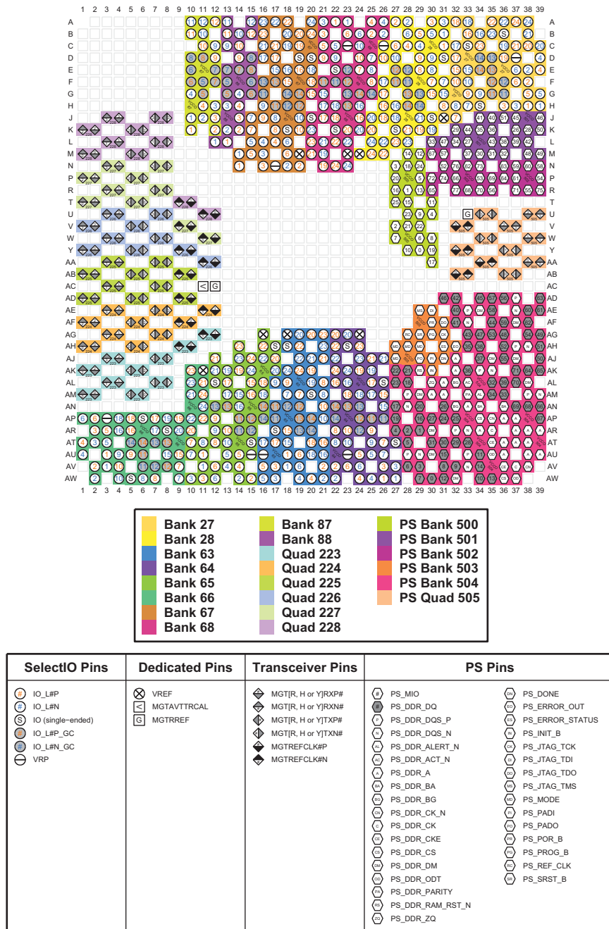
Figure 4-47: FFVF1517 Package—XCZU7EV I/O Bank Diagram
