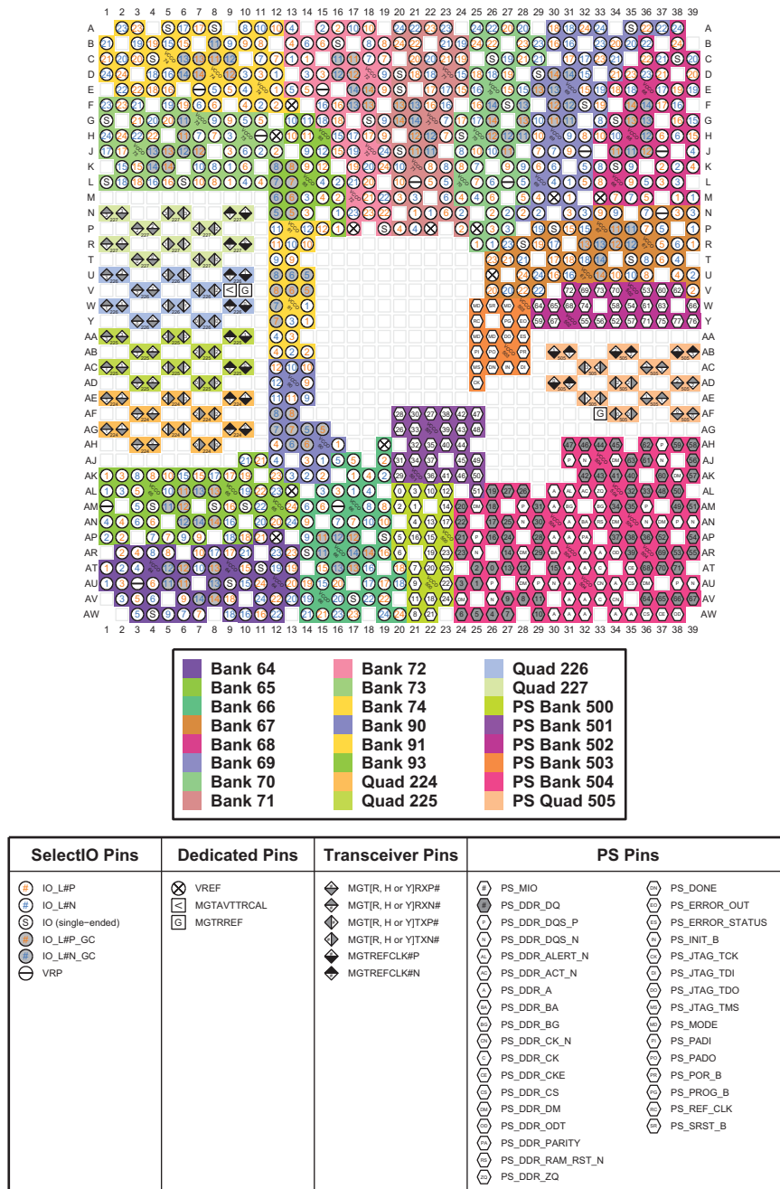
Figure 4-43: FFVB1517 Package—XCZU17EG and XCZU19EG I/O Bank Diagram
