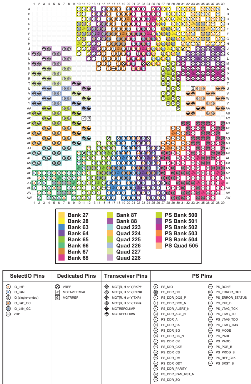
Figure 4-45: FFVF1517 Package—XCZU7CG and XCZU7EG I/O Bank Diagram
