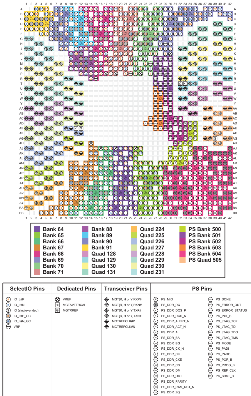
Figure 4-61: FFVC1760 Package—XCZU11EG I/O Bank Diagram
