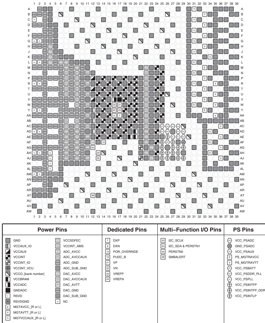
Figure 4-56: FVVG1517 and FSVG1517 Packages—XCZU43DR Power, Dedicated, and Multi-function Pin Diagram
