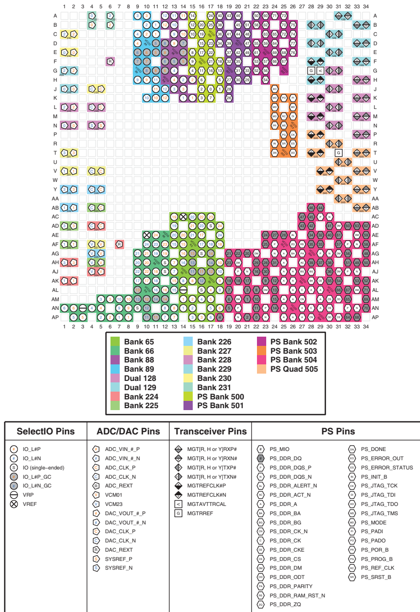
Figure 4-39: FFVE1156 and FSVE1156 Packages—XCZU48DR I/O Bank Diagram
