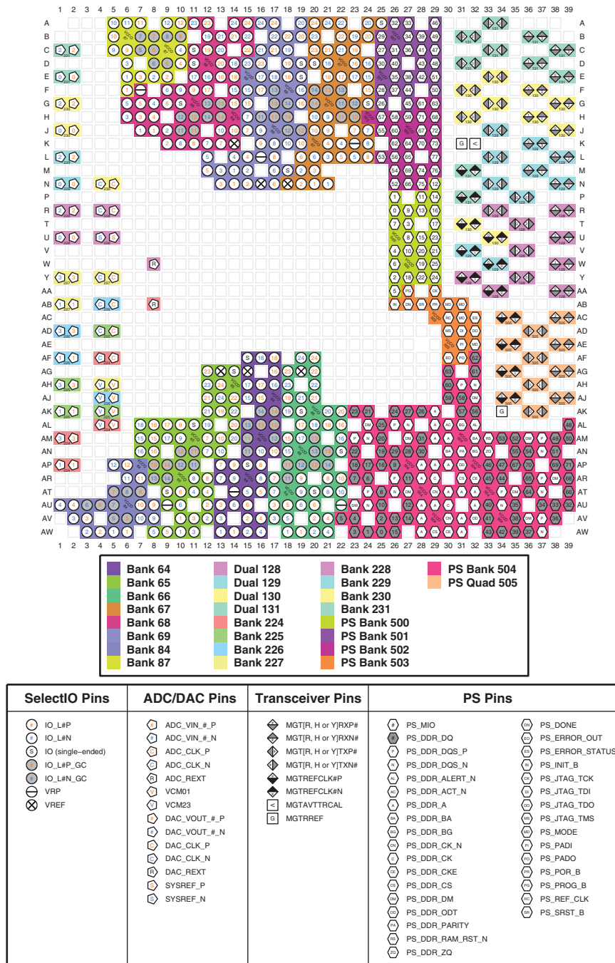
Figure 4-57: FFVG1517 and FSVG1517 Packages—XCZU47DR I/O Bank Diagram
