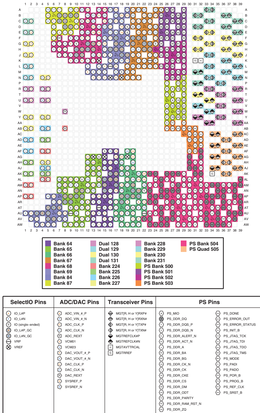
Figure 4-59: FFVG1517 and FSVG1517 Packages—XCZU48DR I/O Bank Diagram
