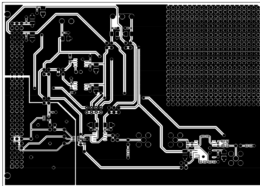
Figure 8. Component Side Artwork
