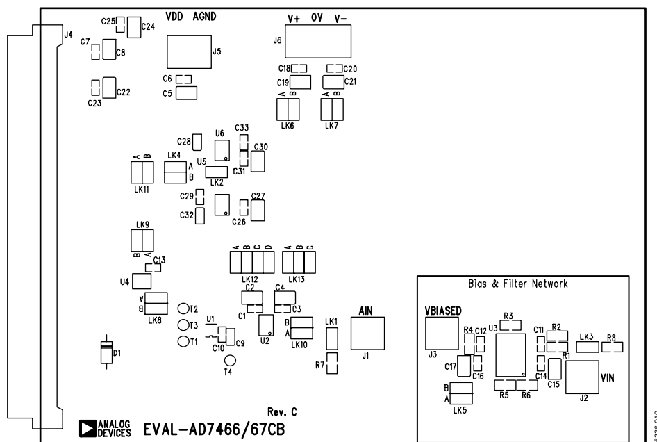
Figure 10. AD7466/AD7467 Evaluation Board Component Placement Drawing
