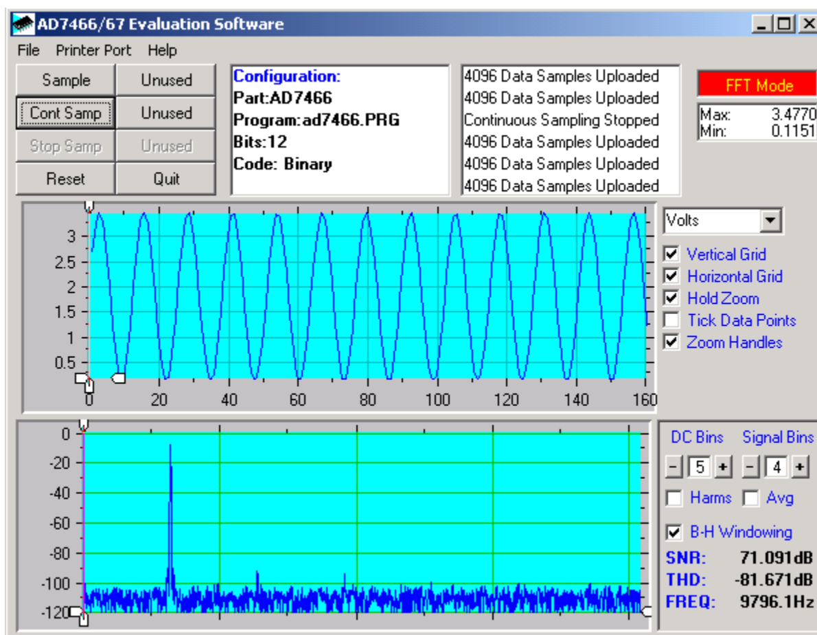
Figure 4. AD7466/AD7467 Evaluation Software, Main Window
