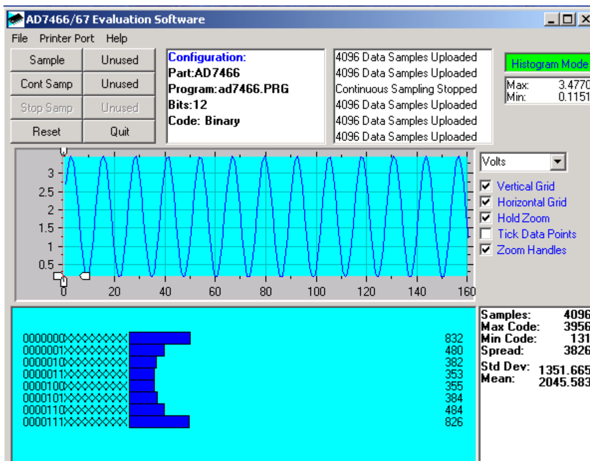
Figure 5. AD7466/AD7467 Evaluation Software, Main Window, Histogram Mode
