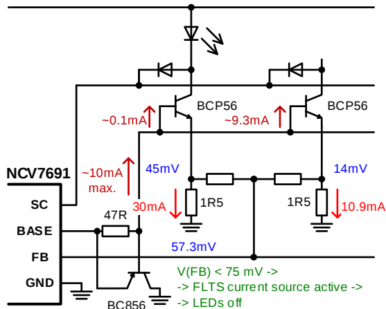
Figure 7: Improved open load detection for 8 strings
