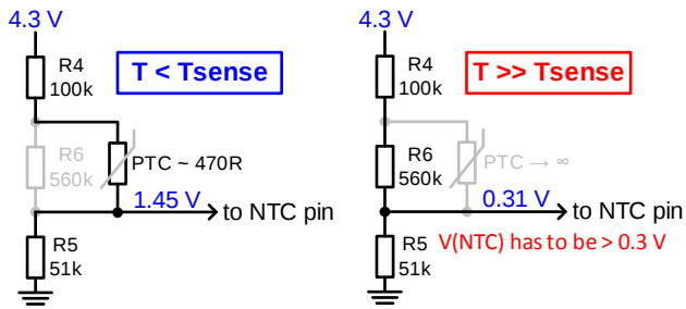
Figure 10: Thermal fold-back circuitry at low / high temperature
