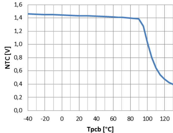
Figure 12: NTC voltage vs. board temperature ( V_S=12\text{V} )
