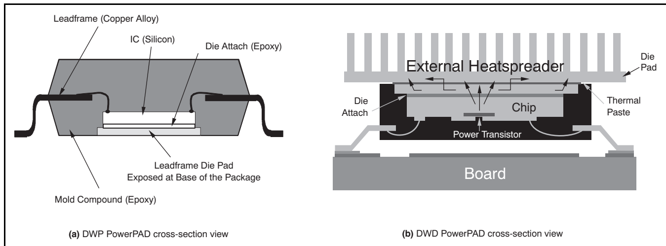
Figure 49. Cross-Section Views
