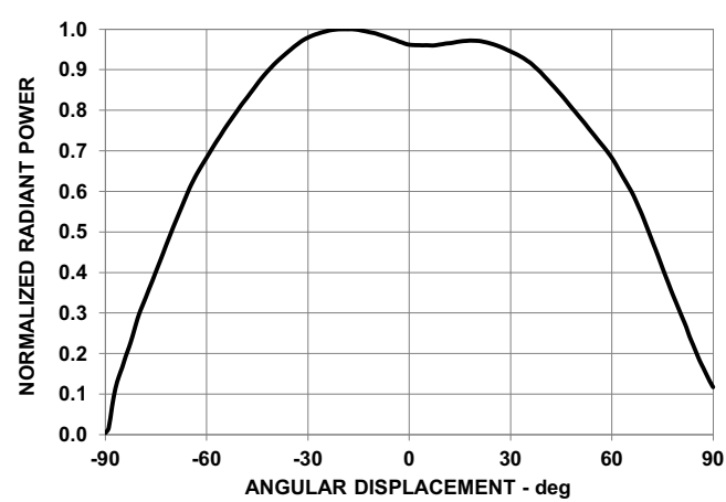
Figure 5: Radiation Pattern
