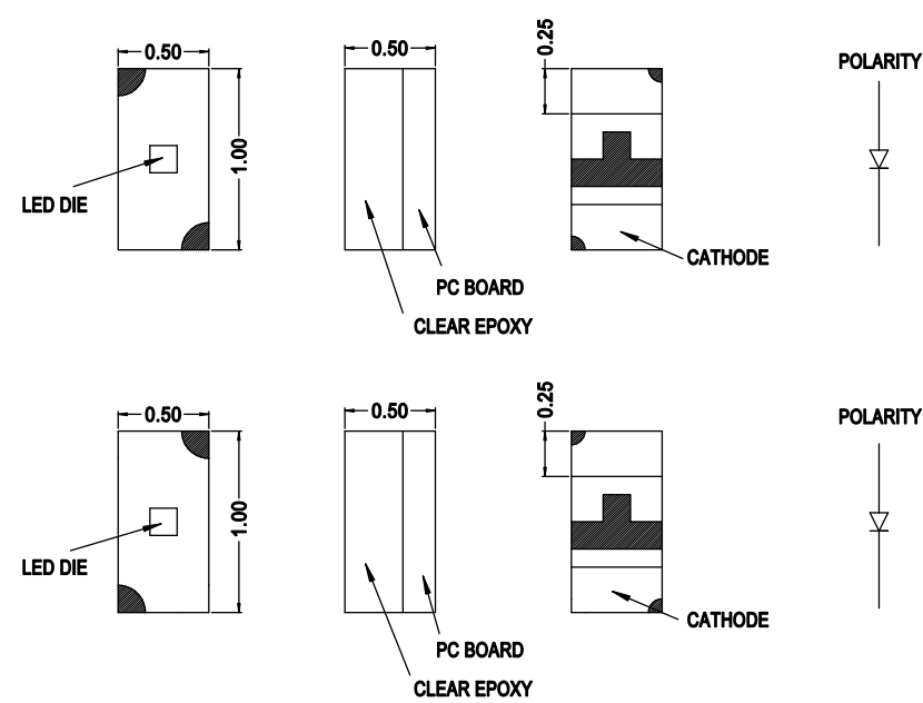
Figure 1: Package Dimensions
