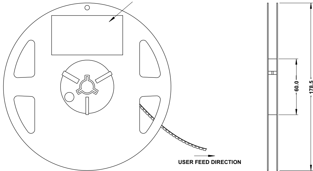
Figure 9: Reel Dimensions
