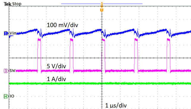
Figure 8. Input Voltage Ripple, I_{OUT} = 1\text{ A}
