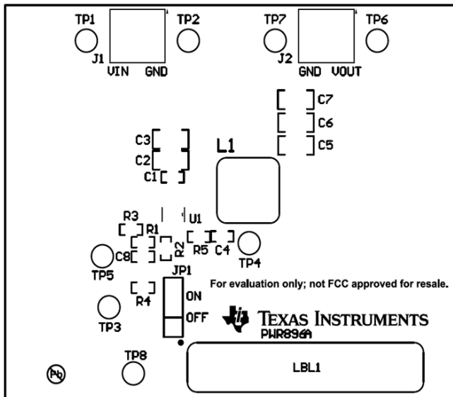
Figure 13. Top Assembly
