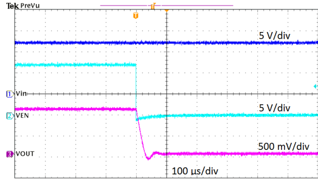
Figure 12. Shut-Down Relative to EN
