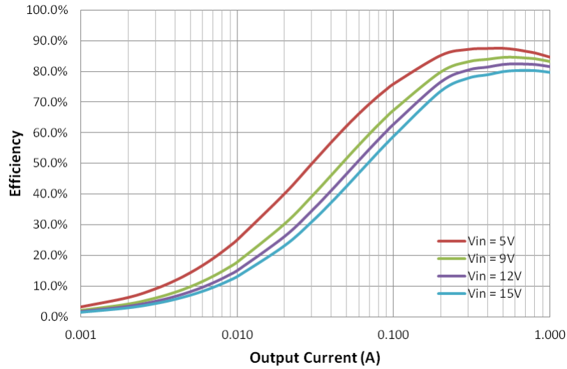
Figure 1. Efficiency
