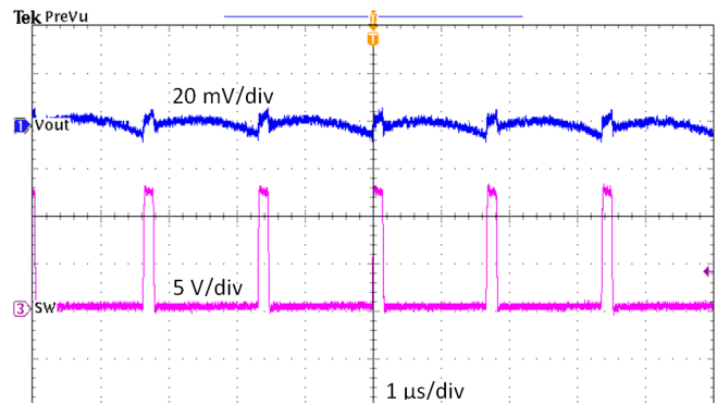
Figure 7. Output Voltage Ripple, I_{OUT} = 0 \text{ A}
