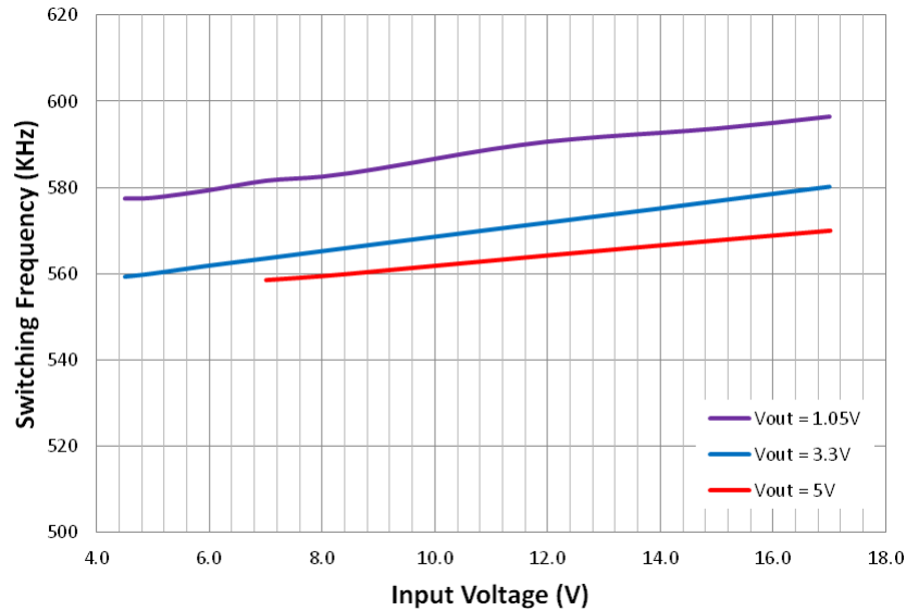
Figure 2. Switching Frequency vs V_{IN}
