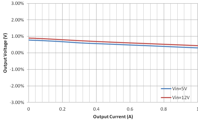
Figure 3. Load Regulation
