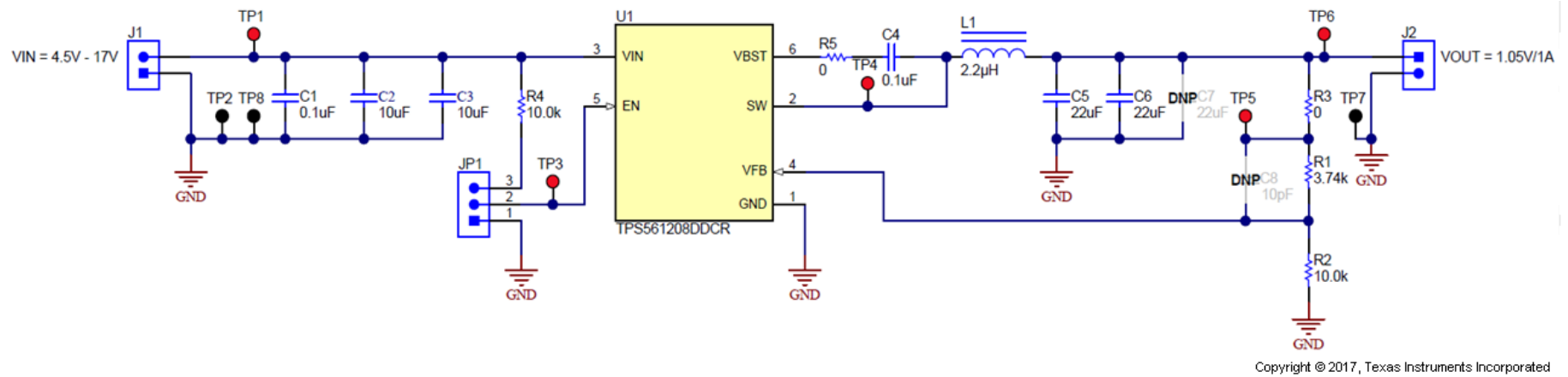
Figure 16. TPS561208EVM-896 Schematic Diagram
