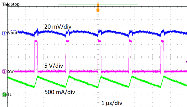
Figure 6. Output Voltage Ripple, I_{OUT} = 1 \text{ A}
