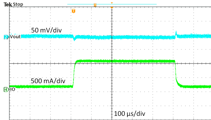
Figure 5. Load Transient Response, 10% to 100% Load Step
