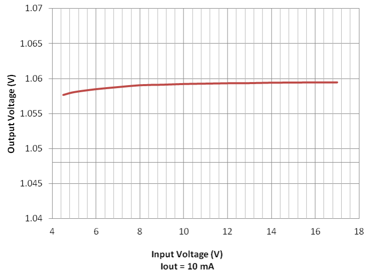
Figure 4. Line Regulation
