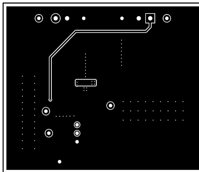
Figure 15. Bottom Layer
