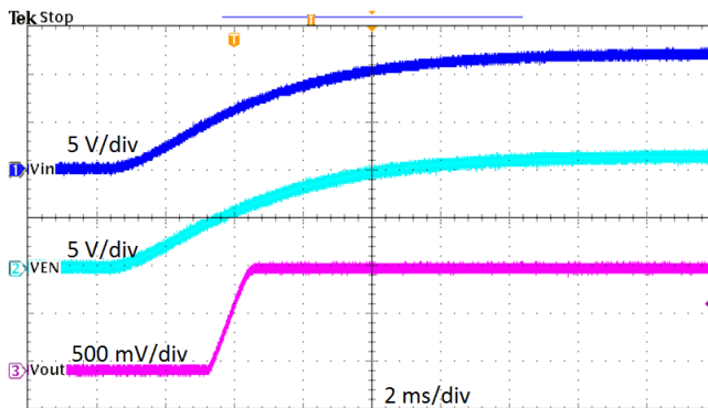
Figure 9. Start-Up Relative to Input Voltage
