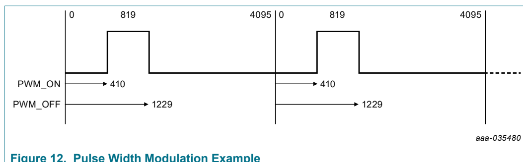
Figure 12. Pulse Width Modulation Example
