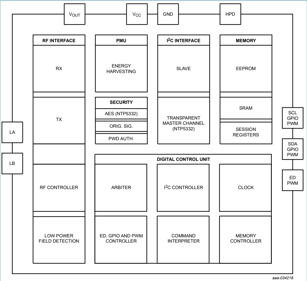
Figure 2. Block diagram NTAG 5 link
