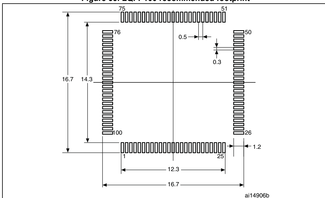
Figure 33. LQFP100 recommended footprint
