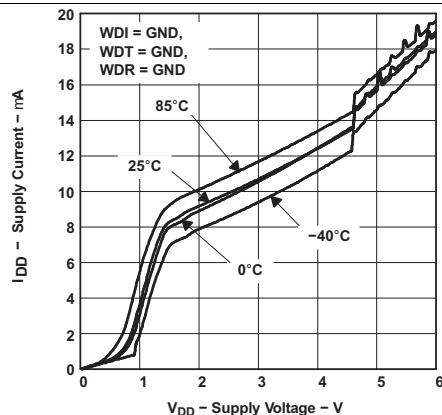
Figure 2. Supply Current vs Supply Voltage
