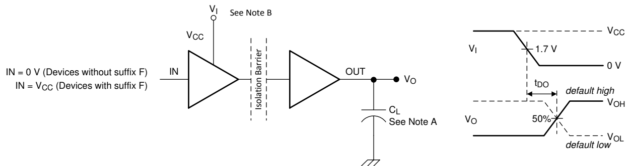
Figure 15. Default Output Delay Time Test Circuit and Voltage Waveforms
