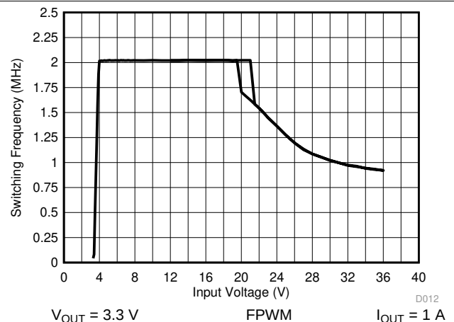
Figure 48. Switching Frequency vs Input Voltage
