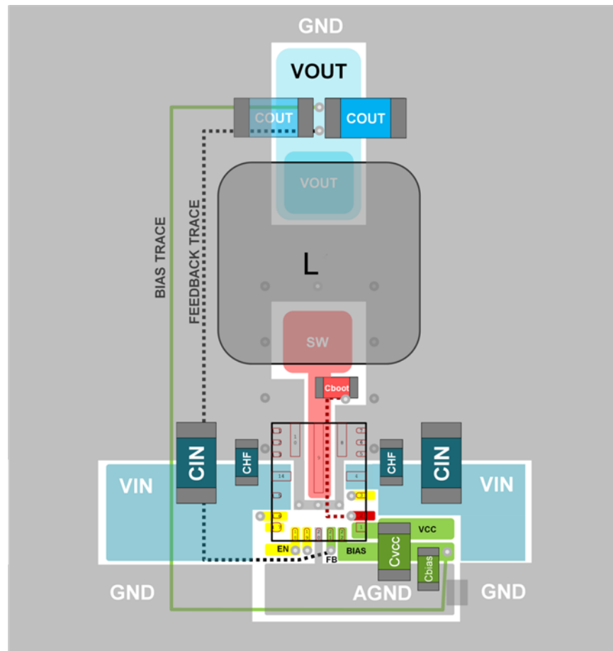
Figure 60. Recommended Layout for LM53625/35-Q1
