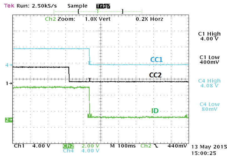
Figure 3. CC Detection
