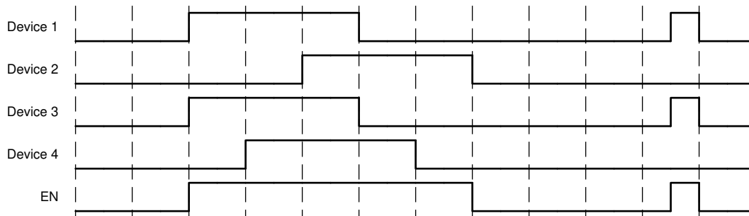
Figure 10. Application timing diagram
