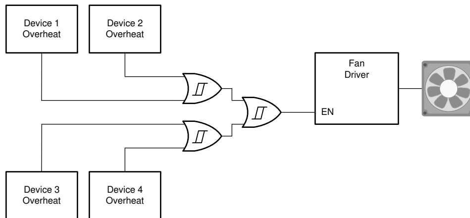
Figure 9. Typical application block diagram
