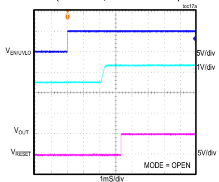
MAX17505S 3.3V OUTPUT SOFT-START WITH 2.5V PREBIAS (PWM MODE, FIGURE 6 CIRCUIT)
