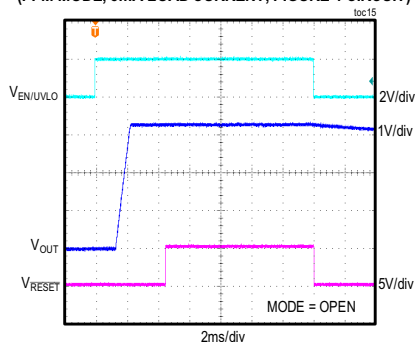
MAX17505 3.3V OUTPUT SOFT-START/SHUTDOWN FROM EN/UVLO (PFM MODE, 5mA LOAD CURRENT, FIGURE 4 CIRCUIT)
