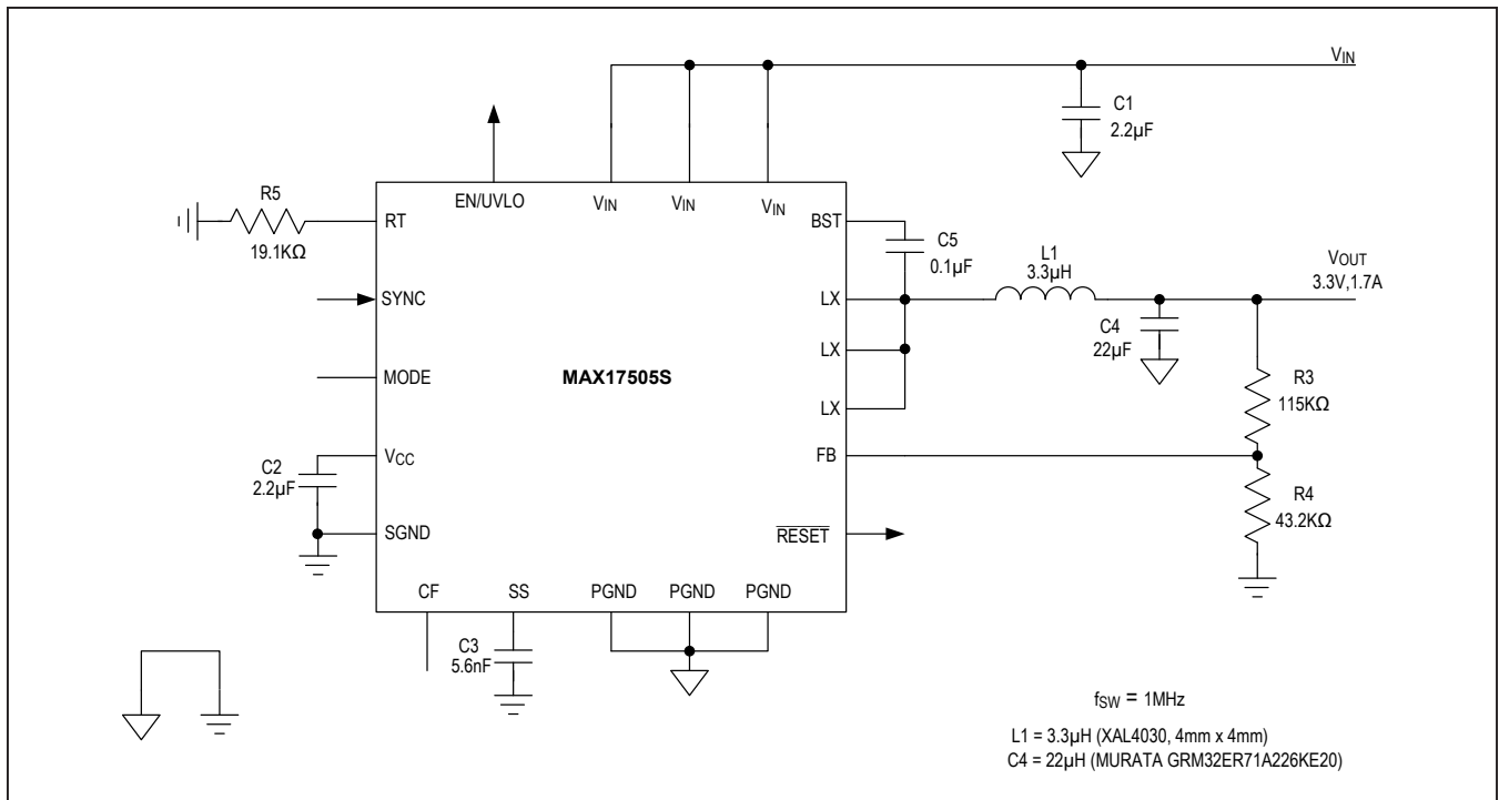
Figure 6. MAX17505S Typical Application Circuit (3.3V Output, 1MHz Switching Frequency)
