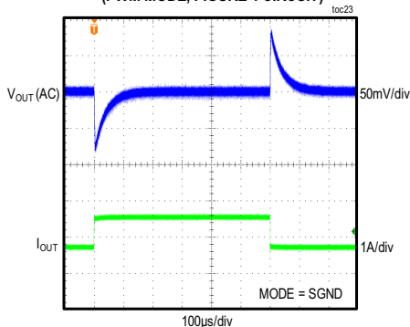
MAX17505 3.3V OUTPUT LOAD CURRENT STEPPED FROM 0.85A TO 1.7A (PWM MODE, FIGURE 4 CIRCUIT)
