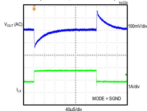
MAX17505S 5V OUTPUT LOAD CURRENT STEPPED FROM 0.85A TO 1A (PWM MODE, FIGURE 5 CIRCUIT)
