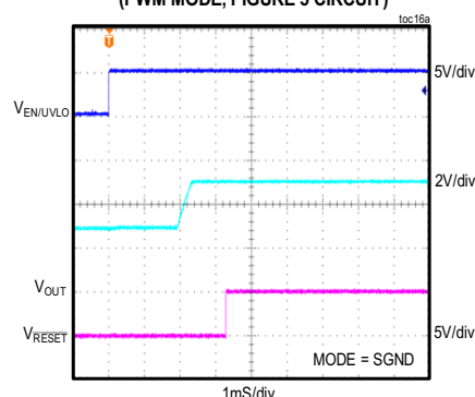
MAX17505S 5V OUTPUT SOFT-START WITH 2.5V PREBIAS (PWM MODE, FIGURE 5 CIRCUIT)
