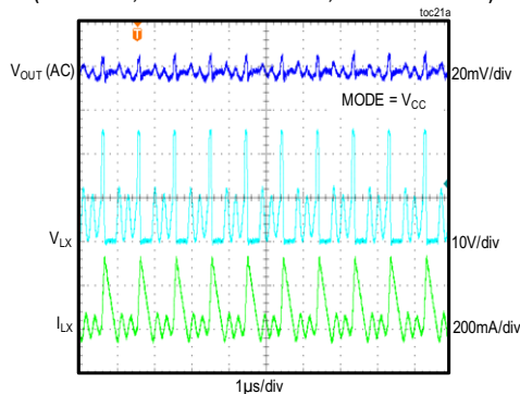
MAX17505S 5V OUTPUT STEADY-STATE SWITCHING WAVEFORMS (DCM MODE, 25mA LOAD CURRENT, FIGURE 5 CIRCUIT)
