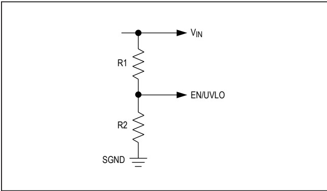
Figure 1. Setting the Input Undervoltage Lockout
