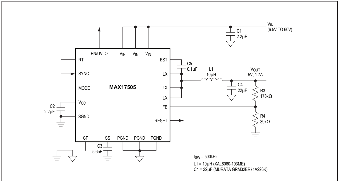
Figure 3. MAX17505 Typical Application Circuit (5V, 500kHz Switching Frequency)
