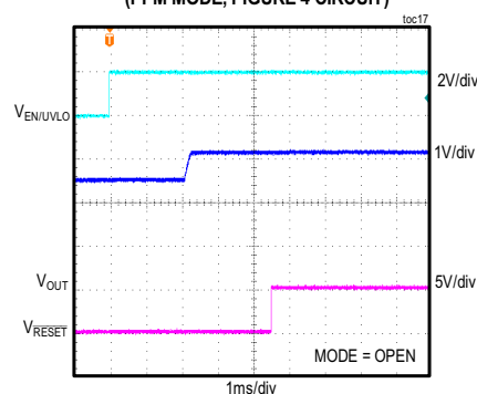
MAX17505 3.3V OUTPUT SOFT-START WITH 2.5V PREBIAS (PFM MODE, FIGURE 4 CIRCUIT)
