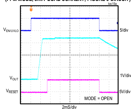
MAX17505S 3.3V OUTPUT SOFT-START/SHUTDOWN FROM EN/UVLO (PFM MODE, 5mA LOAD CURRENT, FIGURE 6 CIRCUIT)
