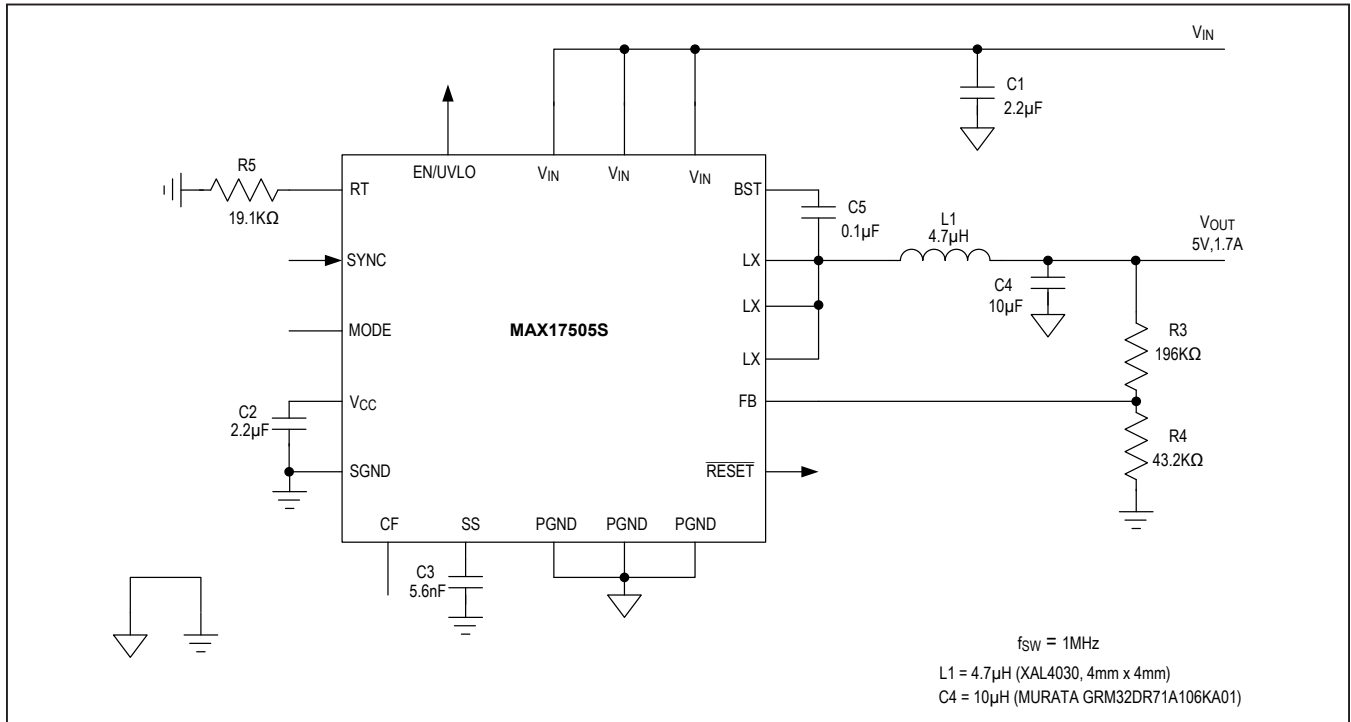
Figure 5. MAX17505S Typical Application Circuit (5V Output, 1MHz Switching Frequency)
