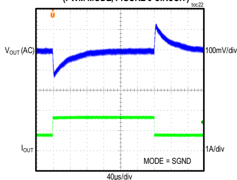
MAX17505 5V OUTPUT LOAD CURRENT STEPPED FROM 0.85A TO 1.7A (PWM MODE, FIGURE 3 CIRCUIT)
