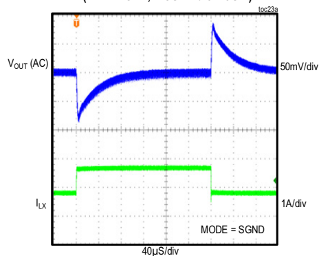
MAX17505S 3.3V OUTPUT LOAD CURRENT STEPPED FROM 0.85A TO 1.7A (PWM MODE, FIGURE 6 CIRCUIT)
