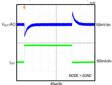
MAX17505 5V OUTPUT LOAD CURRENT STEPPED FROM NO LOAD TO 0.85A (PWM MODE, FIGURE 3 CIRCUIT)
