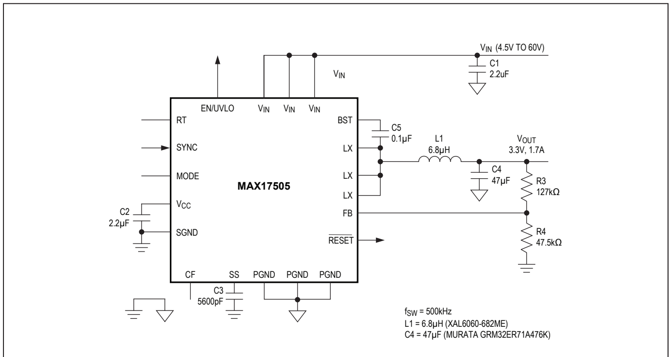
Figure 4. MAX17505 Typical Application Circuit (3.3V, 500kHz Switching Frequency)
