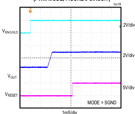
MAX17505 5V OUTPUT SOFT-START WITH 2.5V PREBIAS (PWM MODE, FIGURE 3 CIRCUIT)
