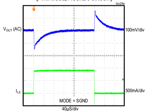
MAX17505S 5V OUTPUT LOAD CURRENT STEPPED FROM NO LOAD TO 0.85A (PWM MODE, FIGURE 5 CIRCUIT)
