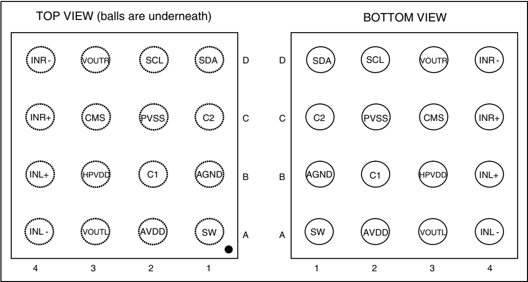
Figure 76. Pinout
