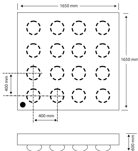
Figure 78. Flip-chip - 16 bumps
