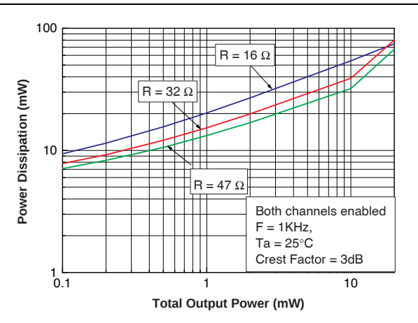
Figure 17. Power dissipation vs. total output power
