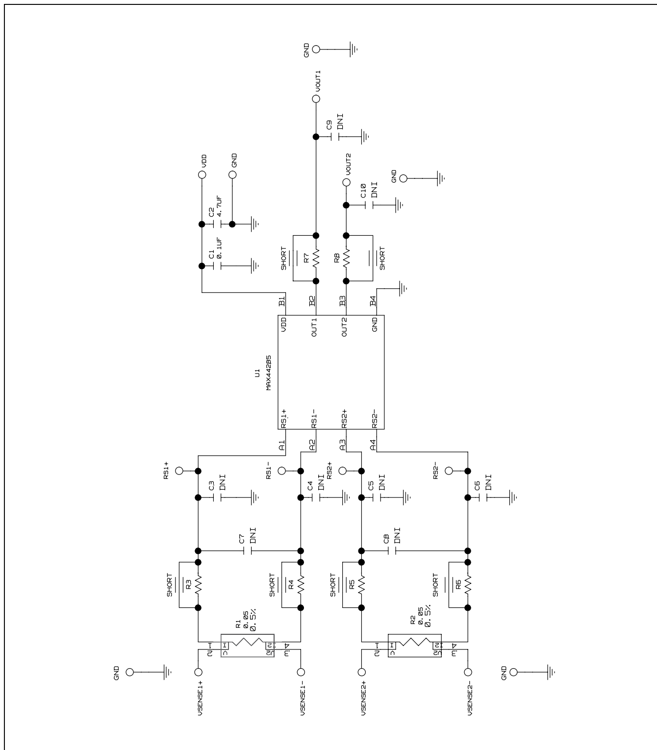
Figure 1. MAX44285 EV Kit Schematic
