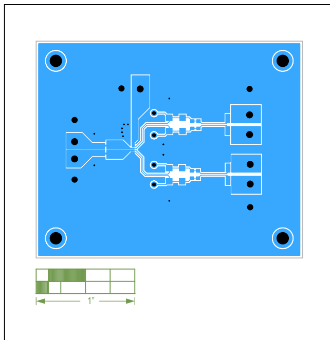
Figure 3. MAX44285 EV Kit PCB Layout—Component Side
