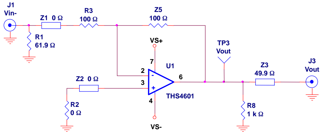
Figure 3-3. DC-Coupled, Dual Power Supply, Inverting Gain Stage
