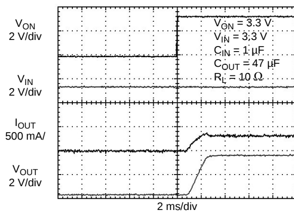
Figure 26. FPF1009 Turn-On Response ( C_{OUT} = 47 \mu F )
