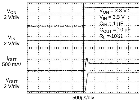
Figure 23. FPF1008 Turn-On Response ( C_{OUT} = 10 \mu F )
