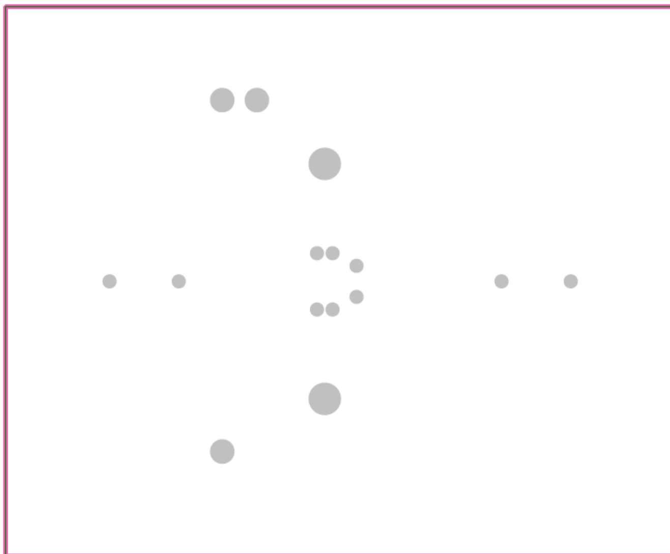
Figure 3. THS4551RGTEVM Layer 2
