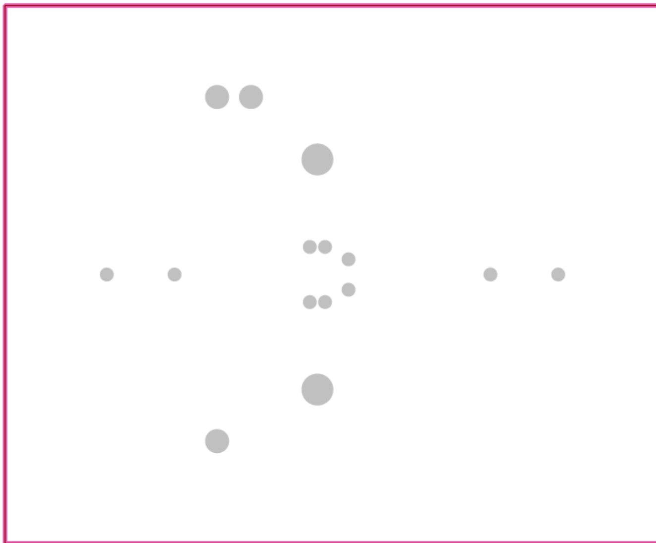
Figure 4. THS4551RGTEVM Layer 3
