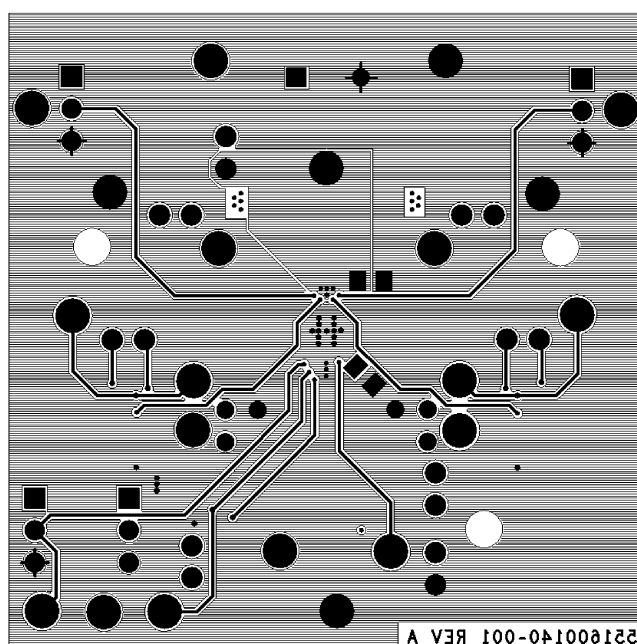
Figure 8. Signal 4 Bottom
