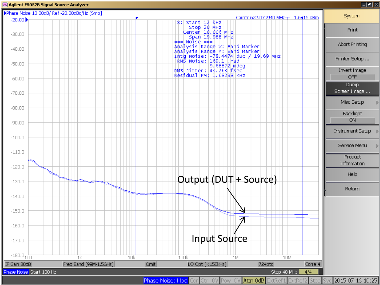
Figure 17. Typical NB7L14 Phase Noise Plot at f_{\text{Carrier}} = 622.08 MHz, V_{\text{CC}} = 3.3 V, 25^{\circ}\text{C}
