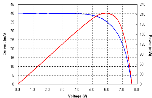
Current-Voltage Characteristics
