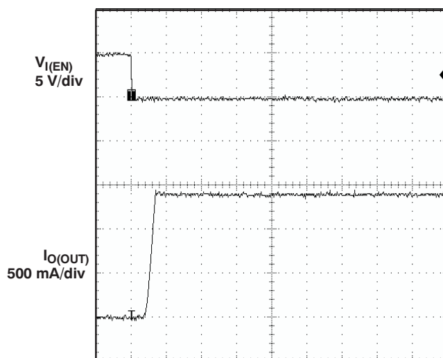
Figure 4. Turnon Delay and Rise Time With 100- \mu F Load
