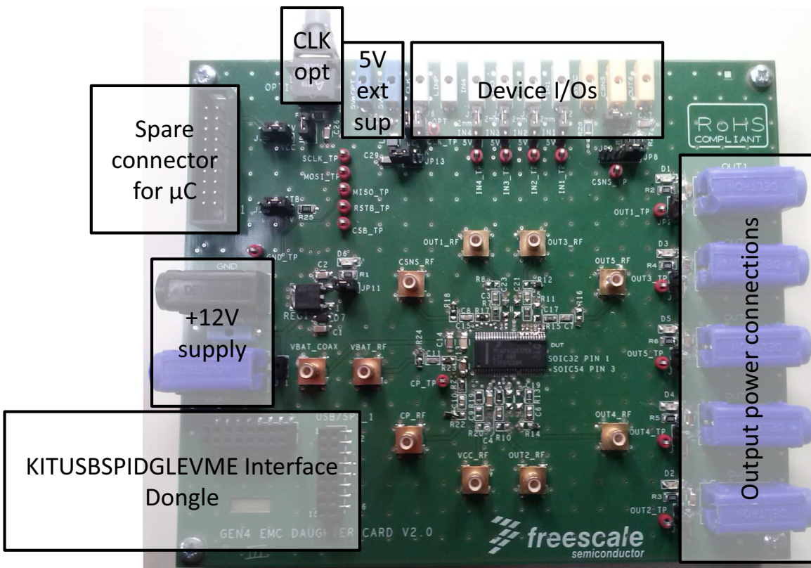
Figure 6. Connector Designations
