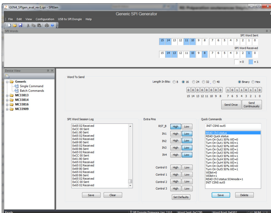
Figure 4. SPIGen GUI
