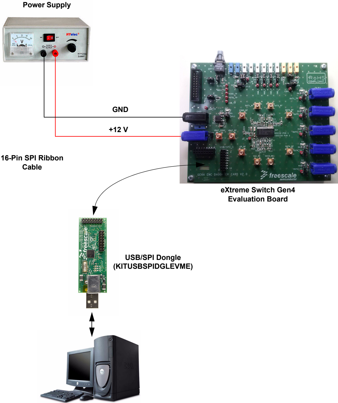
Figure 3. eXtreme Switch Gen4 Evaluation Board plus KITUSBSPIDGLEVME Board Setup
