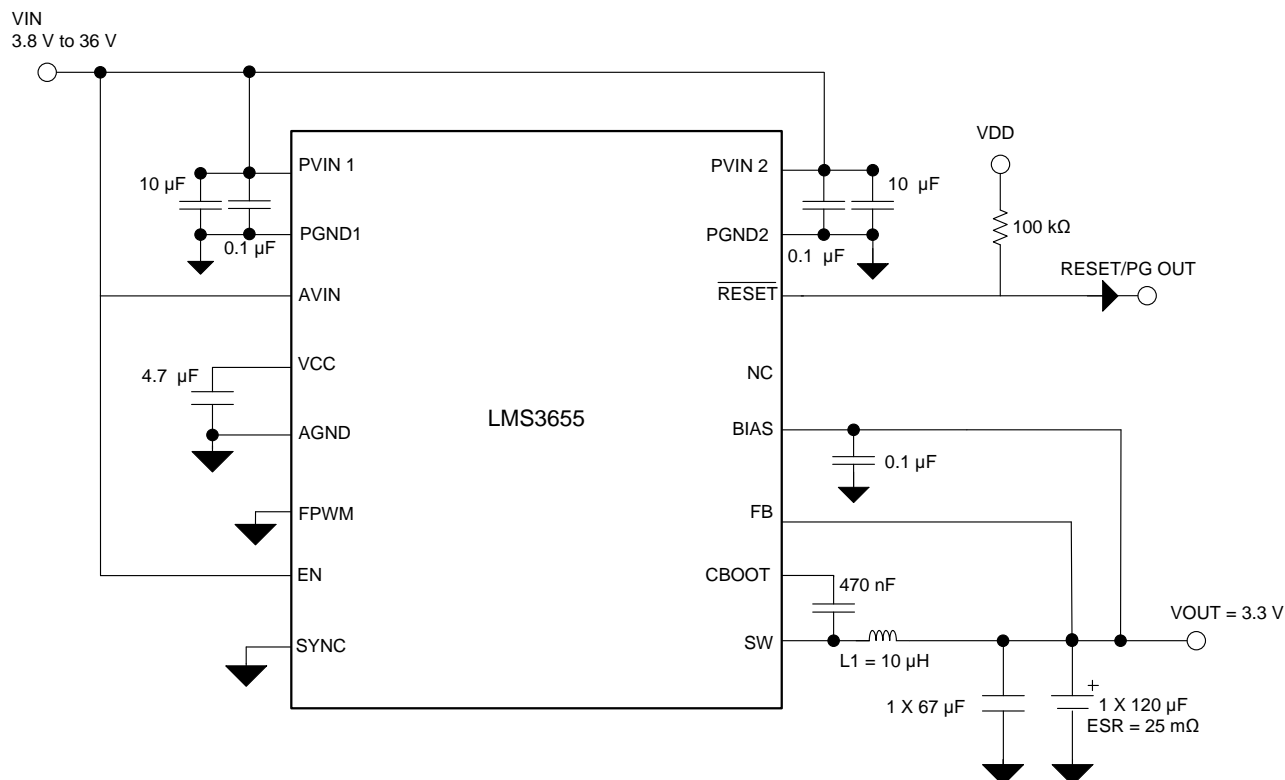
Figure 35. Fixed 3.3-V, 5.5-A Output Power Supply
