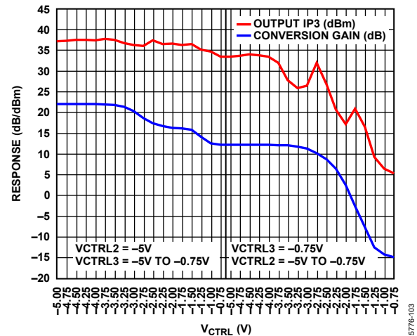
Figure 60. Output IP3 and Conversion Gain vs. V_{CTRL} when VCTRL2 and VCTRL3 Used Separately for Lower Sideband at RFOUT = 18 GHz, T_A = 25^\circ\text{C} , LO = 0 dBm, IF = 3 GHz
