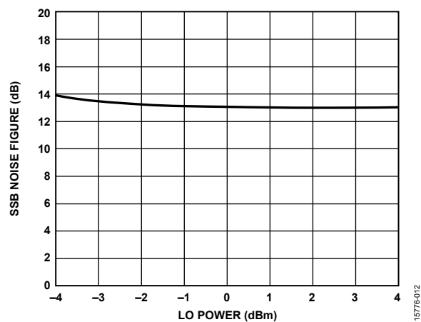
Figure 12. SSB Noise Figure vs. LO Power, RF Frequency = 18 GHz
