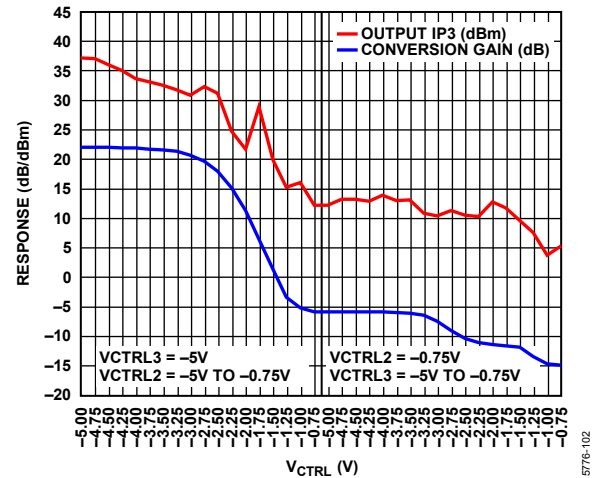
Figure 59. Output IP3 and Conversion Gain vs. V_{CTRL} when VCTRL2 and VCTRL3 Used Separately for Lower Sideband at RFOUT = 18 GHz, T_A = 25^\circ\text{C} , LO = 0 dBm, IF = 3 GHz
