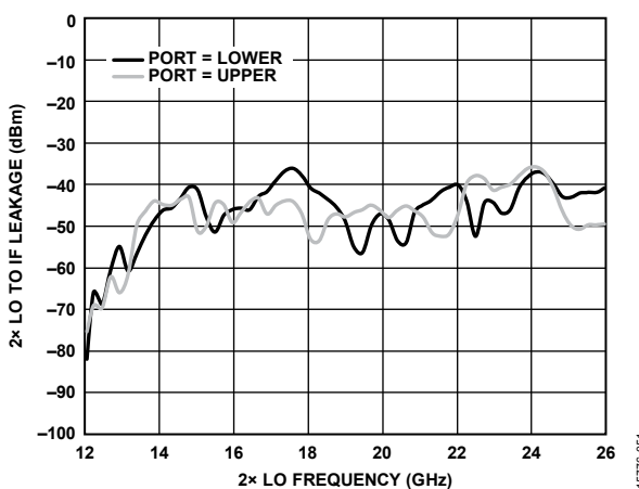
Figure 51. 2x LO to IF Leakage vs. 2x LO Frequency for Upper Sideband and Lower Sideband
