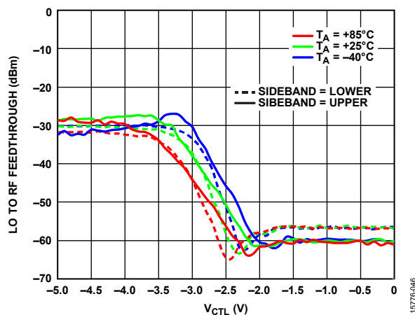
Figure 46. LO to RF Feedthrough vs. V_{CTL} at Various Temperatures and Sidebands, IFx Pin = 0 dBm
