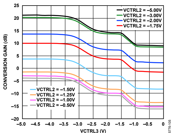
Figure 62. Conversion Gain vs. VCTRL3 at Different VCTRL2 Voltages
