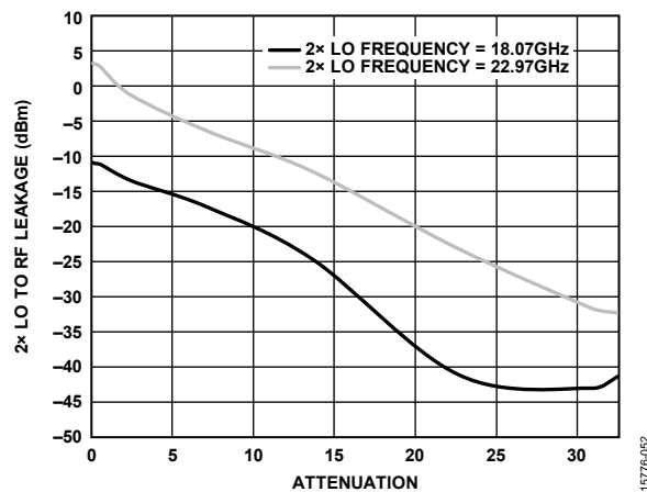
Figure 52. 2x LO to RF Leakage vs. Attenuation for Various Frequencies
