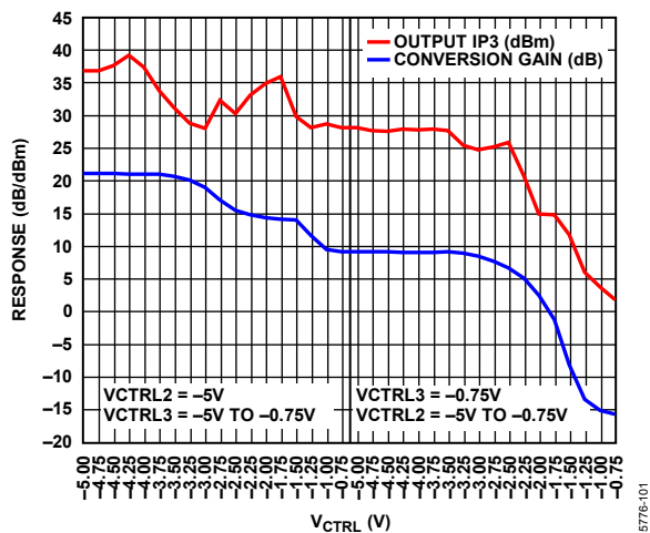
Figure 58. Output IP3 and Conversion Gain vs. V_{CTRL} when VCTRL2 and VCTRL3 Used Separately for Upper Sideband at RFOUT = 23 GHz, T_A = 25^\circ\text{C} , LO = 0 dBm, IF = 3 GHz
