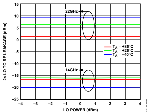
Figure 50. 2x LO to RF Leakage vs. LO Power at Various Temperatures and LO Frequencies, Without Nulling
