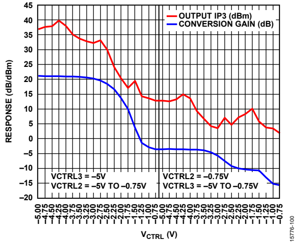
Figure 57. Output IP3 and Conversion Gain vs. V_{CTRL} when VCTRL2 and VCTRL3 Used Separately for the Upper Sideband at RFOUT = 23 GHz, T_A = 25^\circ\text{C} , LO = 0 dBm, IF = 3 GHz
