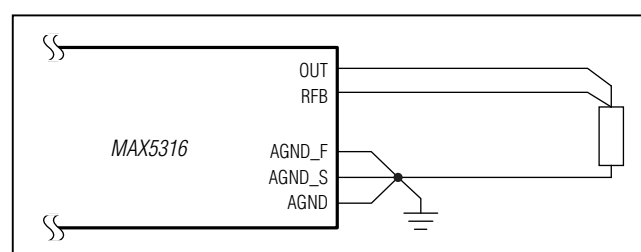
Figure 2a. Star Ground Connection
