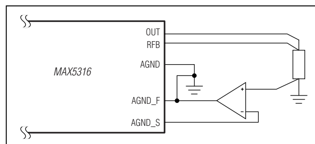
Figure 2b. Force/Sense Connection
