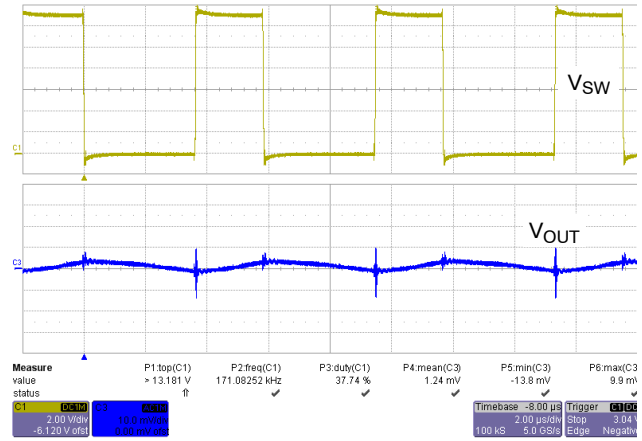
Figure 5. SWN, V_{OUT} at 170 kHz, 13.2 V to 5 V Output
