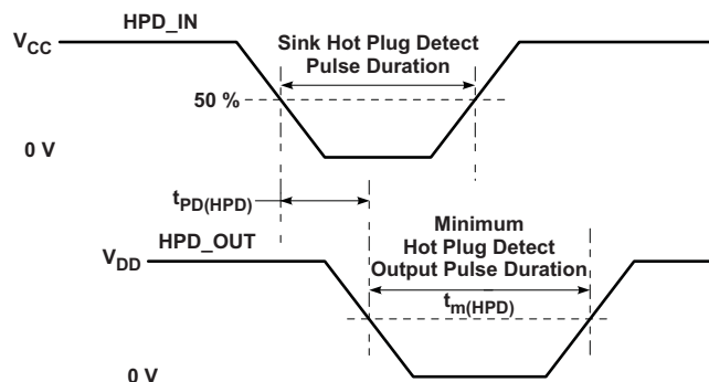
Figure 2. HPD Timing Diagram #1
