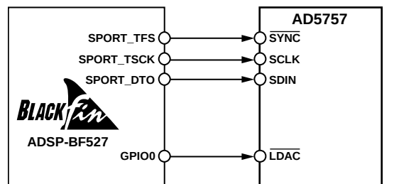
Figure 65. AD5757-to-ADSP-BF527 SPORT Interface
