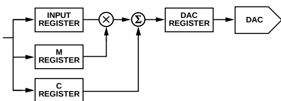
Figure 54. Digital Offset and Gain control
