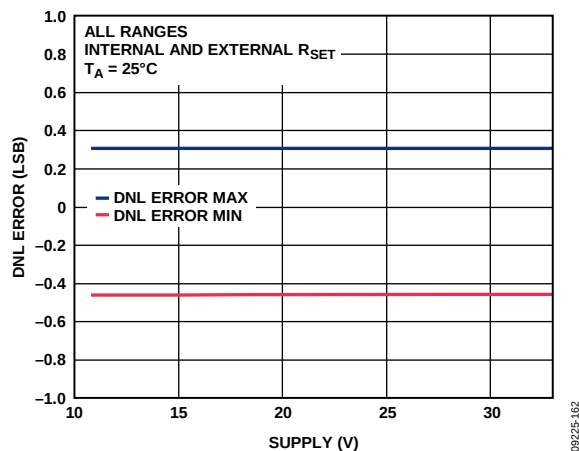
Figure 21. Differential Nonlinearity Error vs. AV_{DD}
