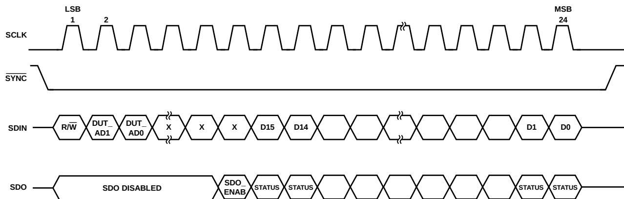
Figure 6. Status Readback During Write
