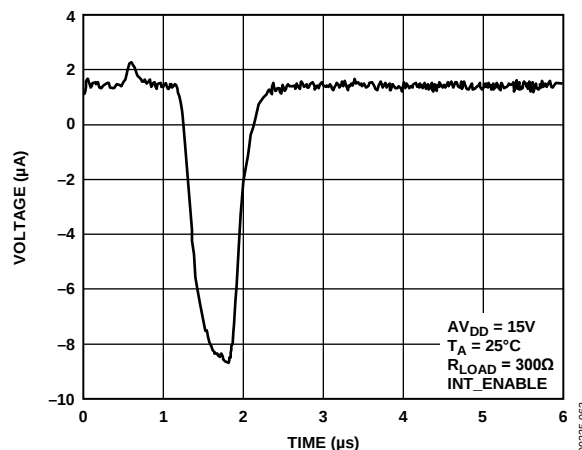
Figure 26. Output Current vs. Time on Output Enable
