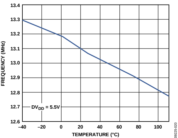
Figure 47. Internal Oscillator Frequency vs. Temperature
