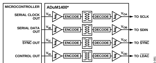
Figure 66. Isolated Interface
