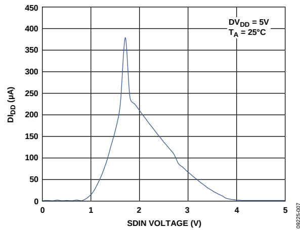
Figure 45. DI_DD vs. Logic Input Voltage
