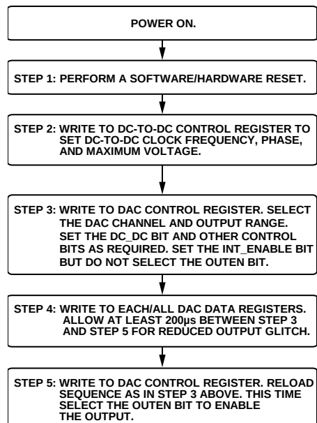
Figure 52. Programming Sequence for Enabling the Output Correctly
