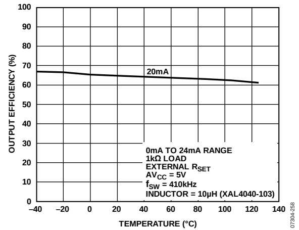
Figure 37. Output Efficiency vs. Temperature (See Figure 57)
