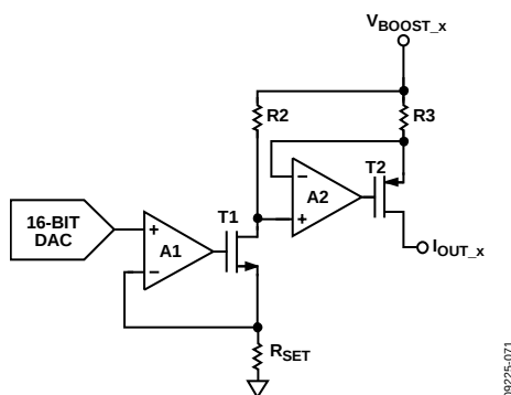
Figure 50. Voltage-to-Current Conversion Circuitry
