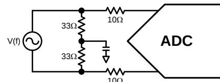
Figure 66. Low-Ω Source, Series 10Ω R, Bandwidth Measurement (Simplified)
